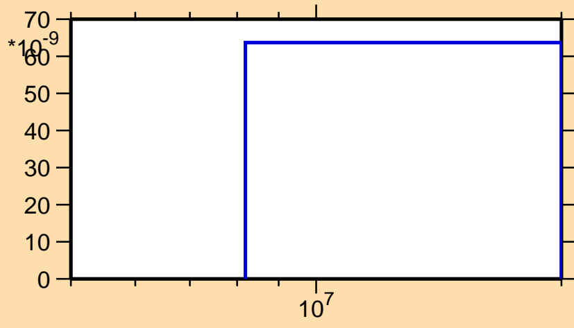
\sigma vs. E for ^{215}\text{Th}(n,\text{nd})
