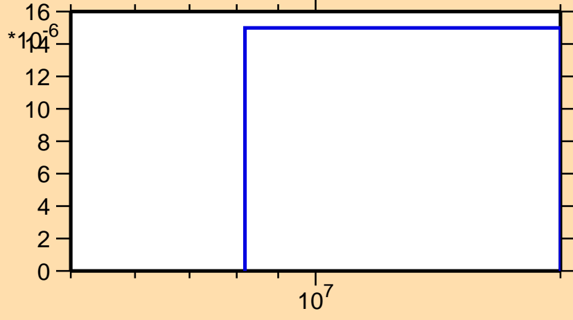
\sigma vs. E for ^{215}\text{Th}(n,3n\alpha)
