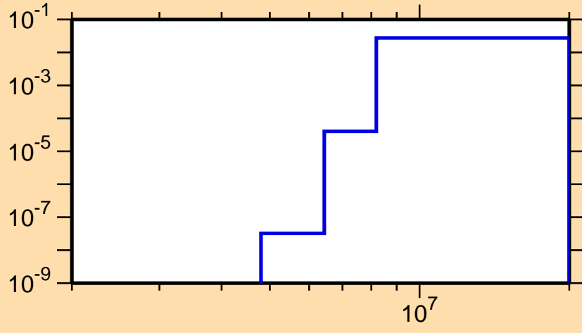
\sigma vs. E for ^{215}\text{Th}(n,np)
