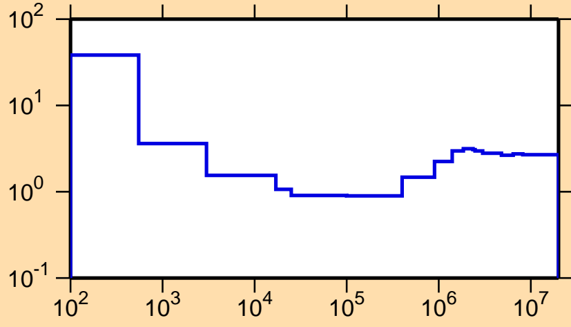
\sigma vs. E for ^{215}\text{Th}(n,\text{nonel.})
