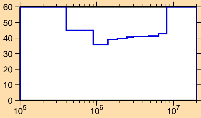
\Delta\sigma/\sigma vs. E for ^{215}\text{Th}(n,n\text{cont.})
