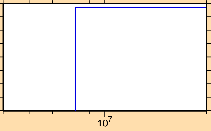
\sigma vs. E for ^{215}\text{Th}(n,2np)
