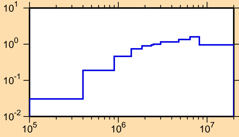
\sigma vs. E for ^{215}\text{Th}(n,n\alpha)
