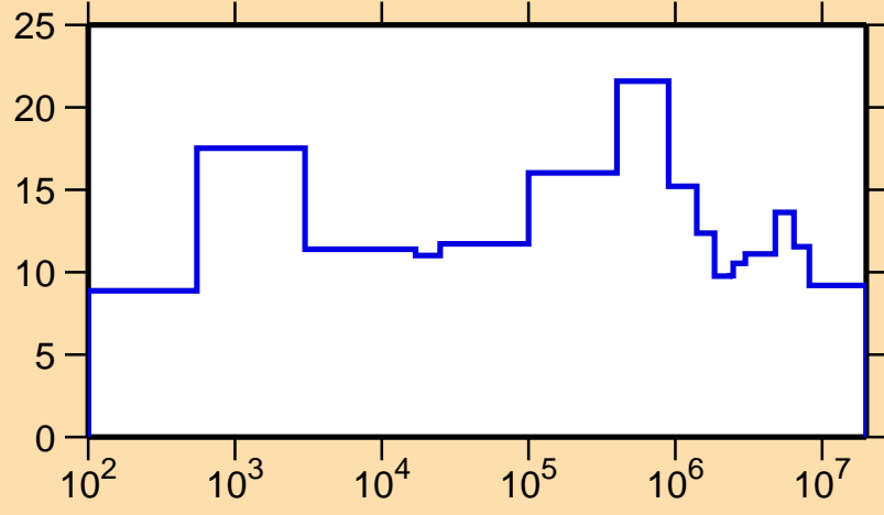
\Delta\sigma/\sigma vs. E for ^{215}\text{Th}(n,el.)
