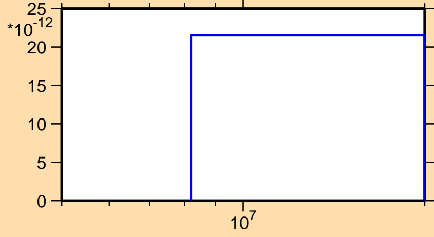
\sigma vs. E for ^{215}\text{Th}(n,nt)
