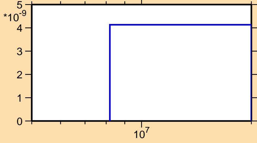
\sigma vs. E for ^{215}\text{Th}(n,pd)
