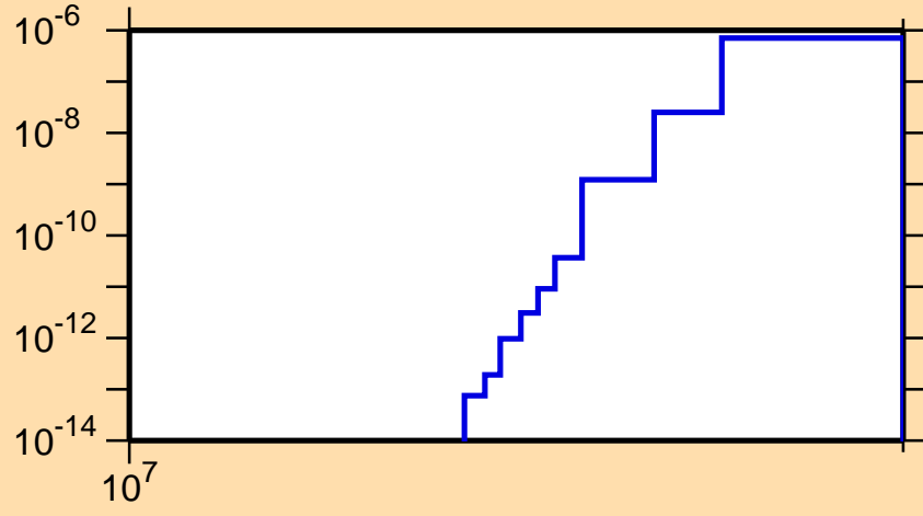
\sigma vs. E for ^{224}\text{Th}(n,nd)
