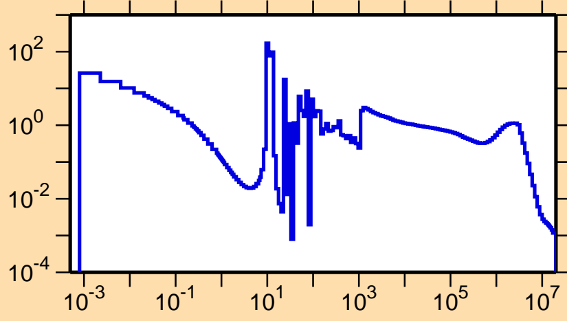
\sigma vs. E for ^{224}\text{Th}(n,\gamma)
