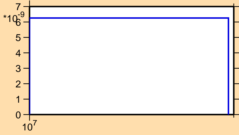
\sigma vs. E for ^{224}\text{Th}(n,nt)
