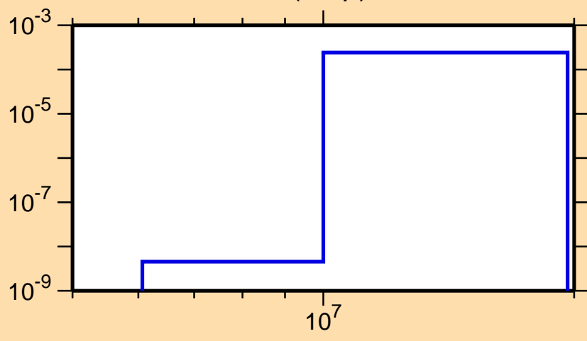
\sigma vs. E for ^{224}\text{Th}(n,np)
