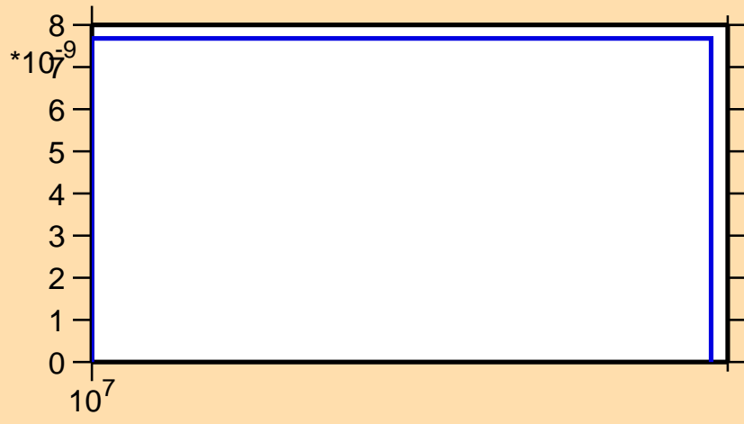
\sigma vs. E for ^{224}\text{Th}(n,\text{nd})
