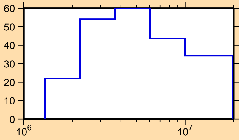
\Delta\sigma/\sigma vs. E for ^{224}\text{Th}(n,p)
