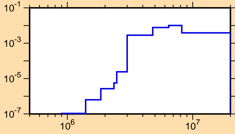
\sigma vs. E for ^{224}\text{Th}(n,n\alpha)
