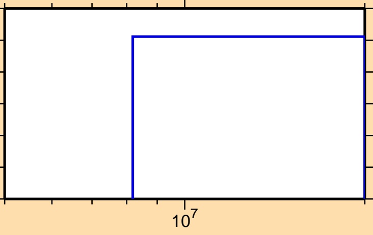
\sigma vs. E for ^{224}\text{Th}(n,2np)
