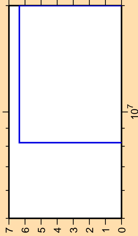
\Delta\sigma/\sigma vs. E for ^{224}\text{Th}(n,nt)
