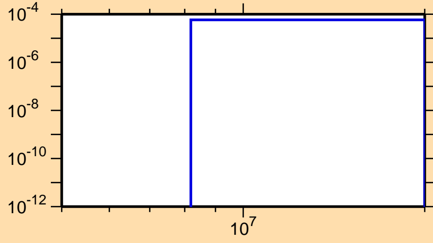
\sigma vs. E for ^{224}\text{Th} (mt 45)
