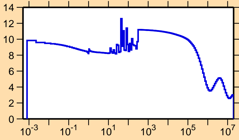
\sigma vs. E for ^{225}\text{Th}(n,\text{el.})
