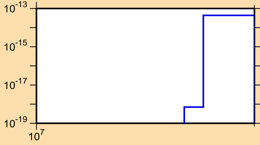
\sigma vs. E for ^{225}\text{Th} (mt 11)
