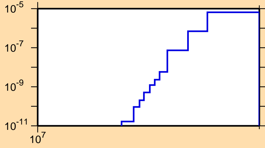
\sigma vs. E for ^{225}\text{Th}(n,\text{nd})
