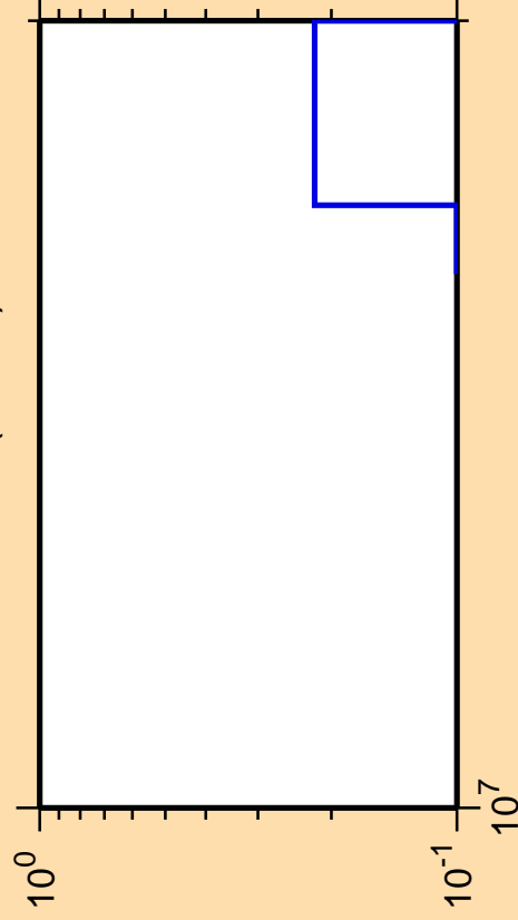
\Delta\sigma/\sigma vs. E for ^{225}\text{Th} (mt 11)
