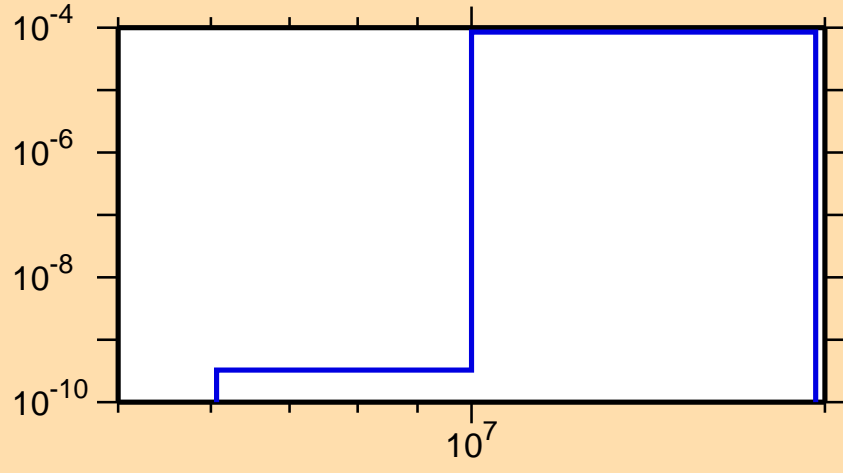
\sigma vs. E for ^{225}\text{Th}(\text{mt117})
