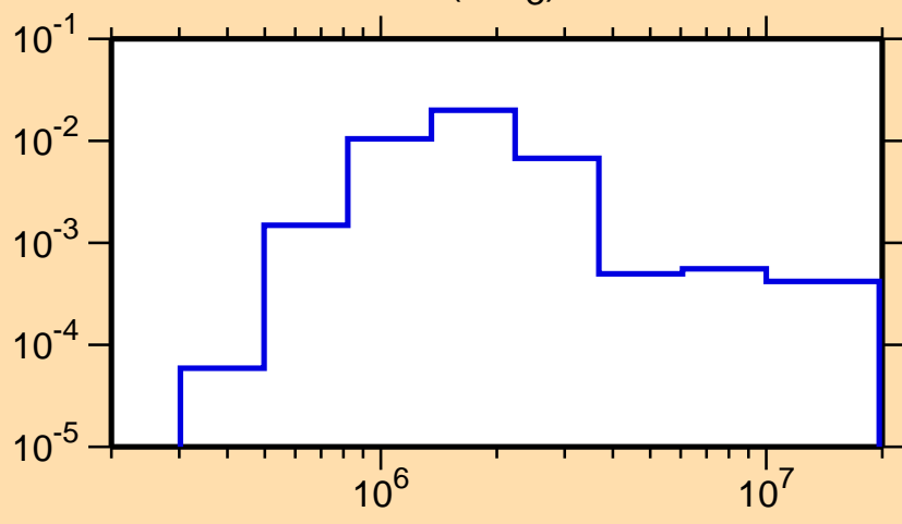
\sigma vs. E for ^{225}\text{Th}(n,n_3)
