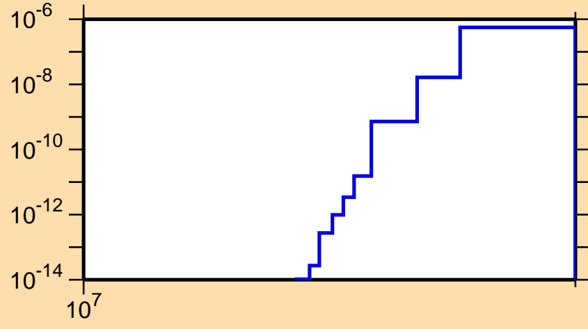
\sigma vs. E for ^{226}\text{Th}(n,\text{nd})
