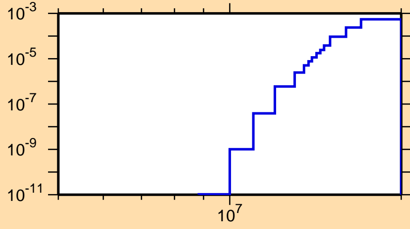
\sigma vs. E for ^{226}\text{Th}(n,t)
