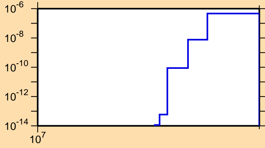
\sigma vs. E for ^{226}\text{Th}(n,2np)
