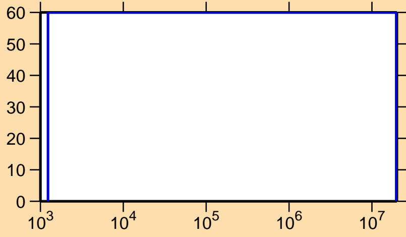
\Delta\sigma/\sigma vs. E for ^{226}\text{Th}(n,\gamma)
