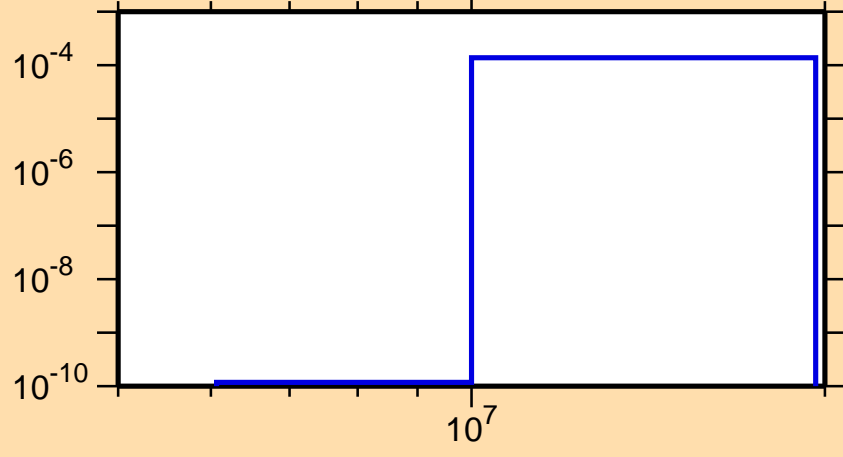
\sigma vs. E for ^{226}\text{Th}(n,np)
