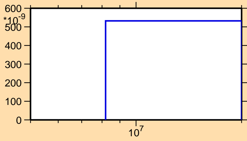
\sigma vs. E for ^{226}\text{Th}(\text{mt117})
