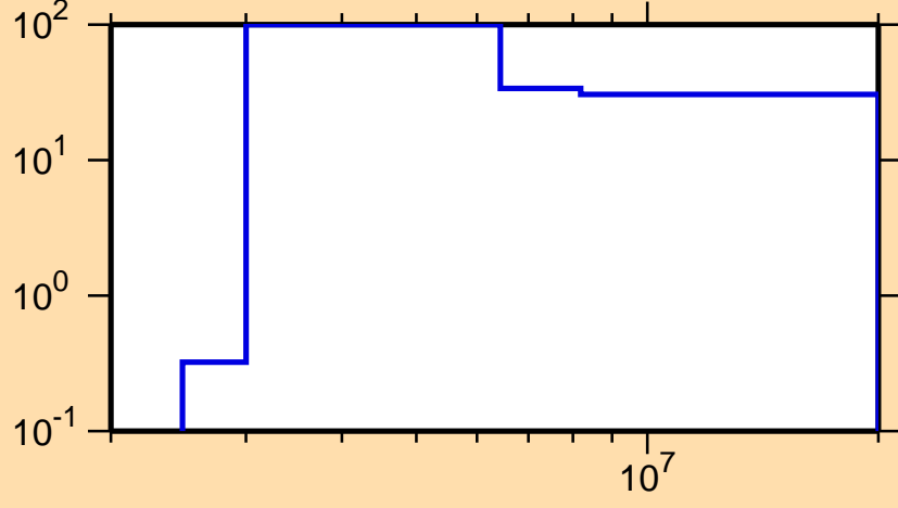
\Delta\sigma/\sigma vs. E for ^{226}\text{Th}(n,p)
