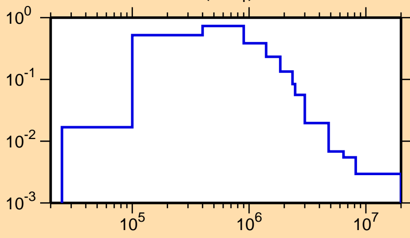
\sigma vs. E for ^{226}\text{Th}(n,n_1)
