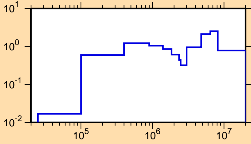
\sigma vs. E for ^{226}\text{Th}(n,\text{inel.})
