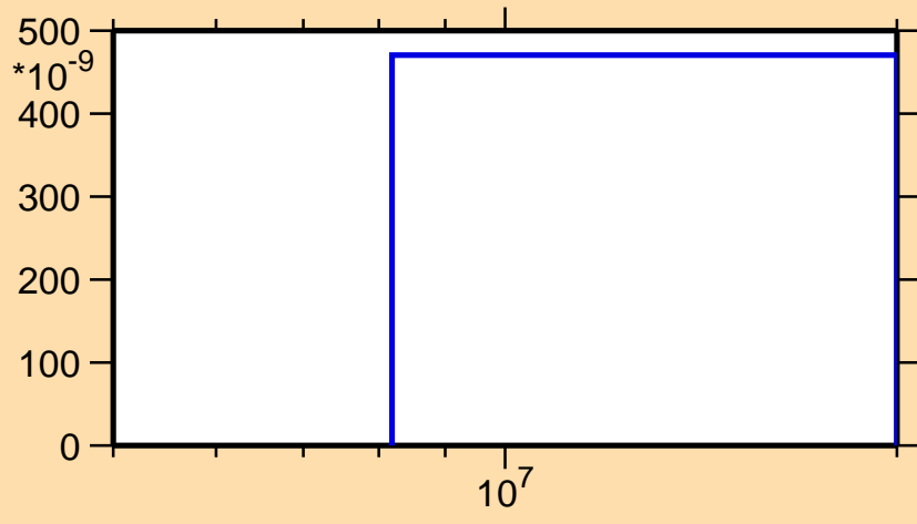
\sigma vs. E for ^{226}\text{Th}(\text{mt } 45)
