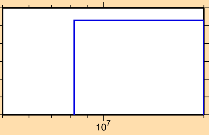
\sigma vs. E for ^{226}\text{Th}(n,\text{nd})
