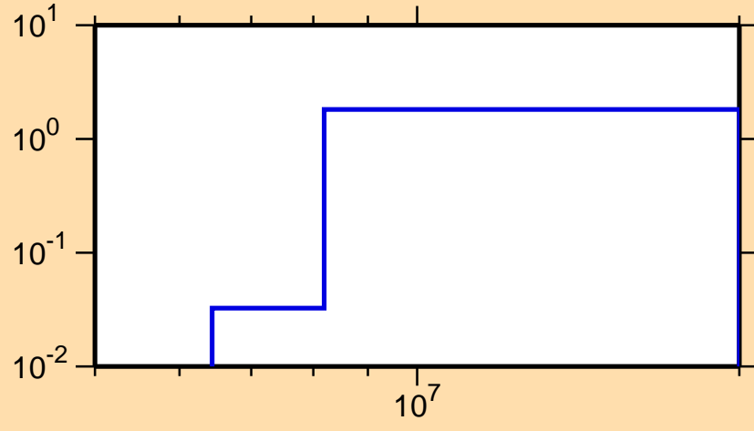
\sigma vs. E for ^{226}\text{Th}(n,2n)
