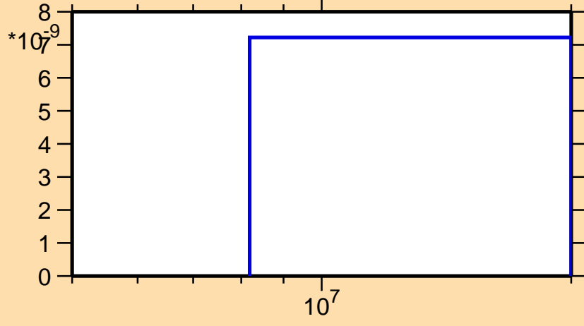
\sigma vs. E for ^{226}\text{Th}(n,nt)
