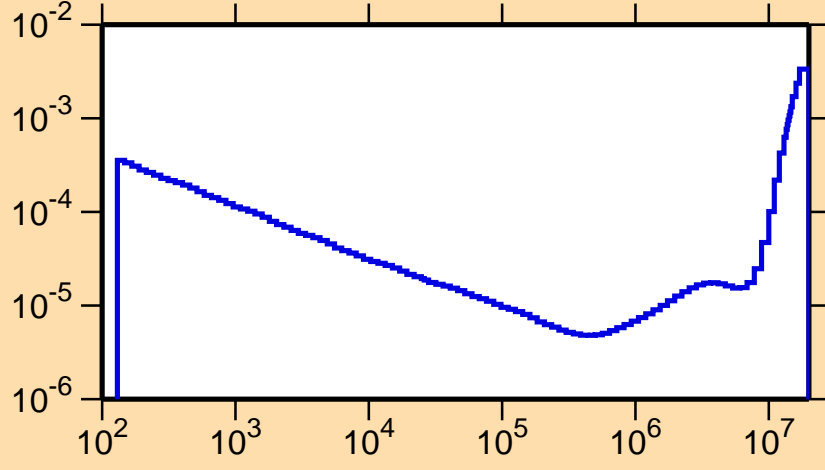
\sigma vs. E for ^{227}\text{Th}(n,\alpha)
