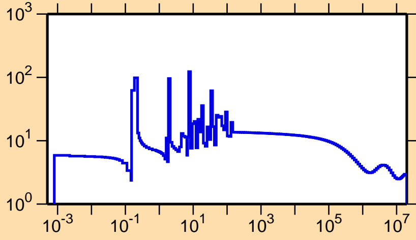
\sigma vs. E for ^{227}\text{Th}(n,\text{el.})
