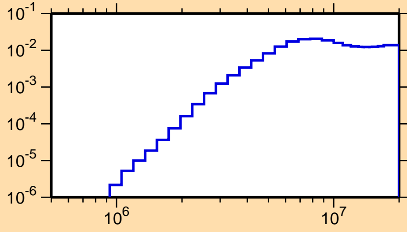
\sigma vs. E for ^{227}\text{Th}(n,n\alpha)
