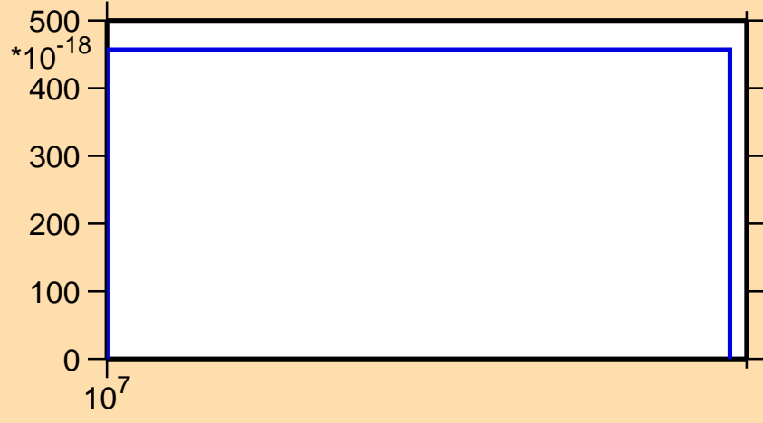
\sigma vs. E for ^{227}\text{Th} (mt 11)
