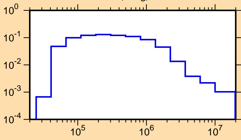
\sigma vs. E for ^{227}\text{Th}(n,n_3)
