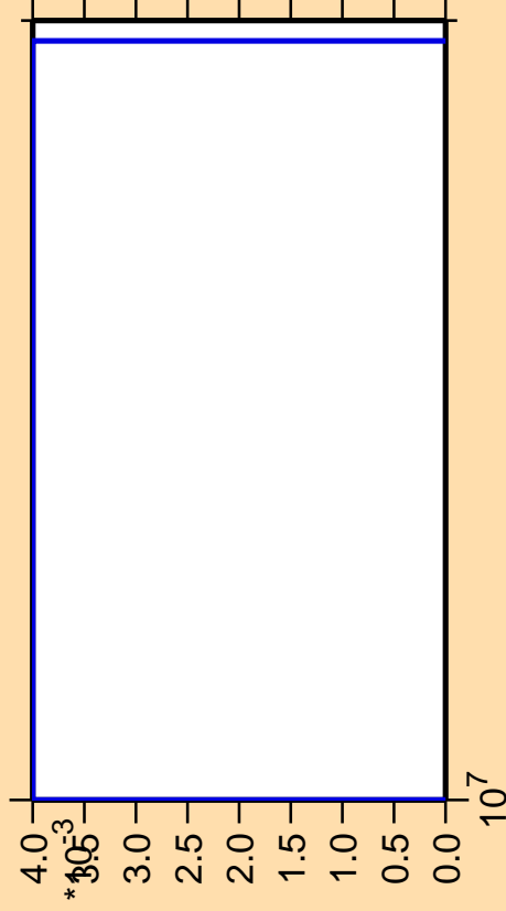
\Delta\sigma/\sigma vs. E for ^{227}\text{Th} (mt 11)
