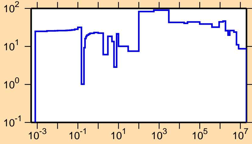
\Delta\sigma/\sigma vs. E for ^{227}\text{Th}(n,el.)
