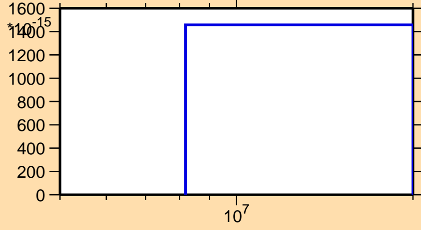
\sigma vs. E for ^{227}\text{Th}(\text{mt117})
