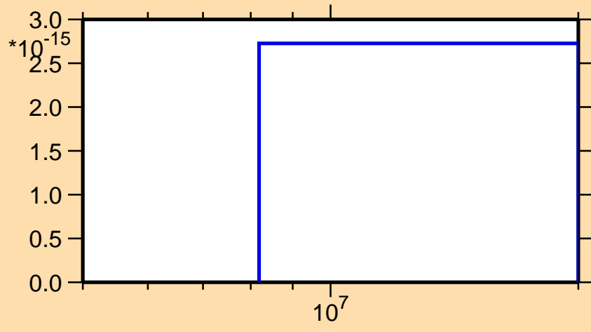
\sigma vs. E for ^{227}\text{Th} (mt 34)
