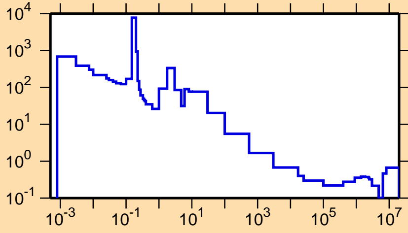
\sigma vs. E for ^{227}\text{Th}(n,f)
