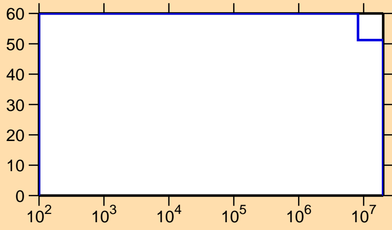
\Delta\sigma/\sigma vs. E for ^{227}\text{Th}(n,\gamma)
