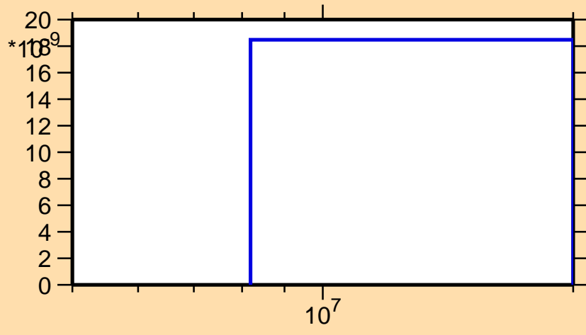
\sigma vs. E for ^{227}\text{Th}(n,nt)
