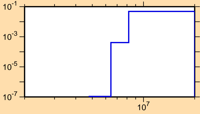
\sigma vs. E for ^{227}\text{Th}(n,2n\alpha)
