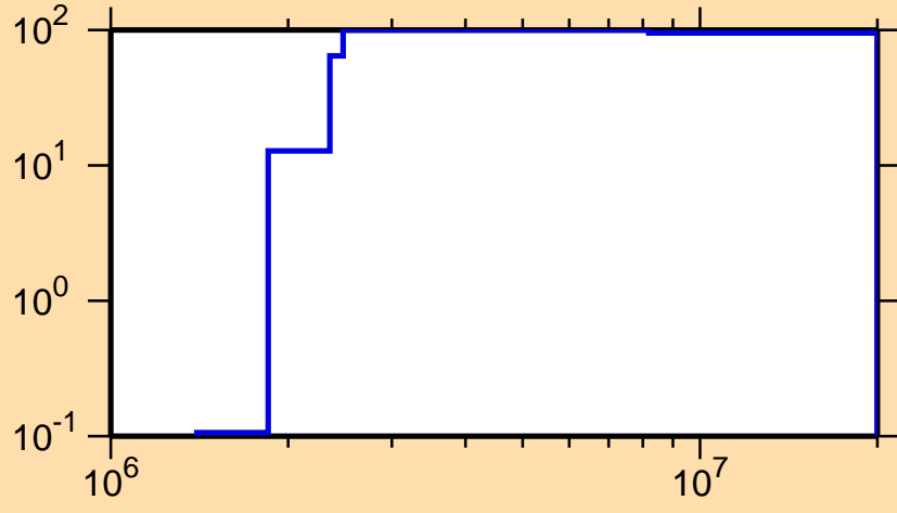
\Delta\sigma/\sigma vs. E for ^{227}\text{Th}(n,p)
