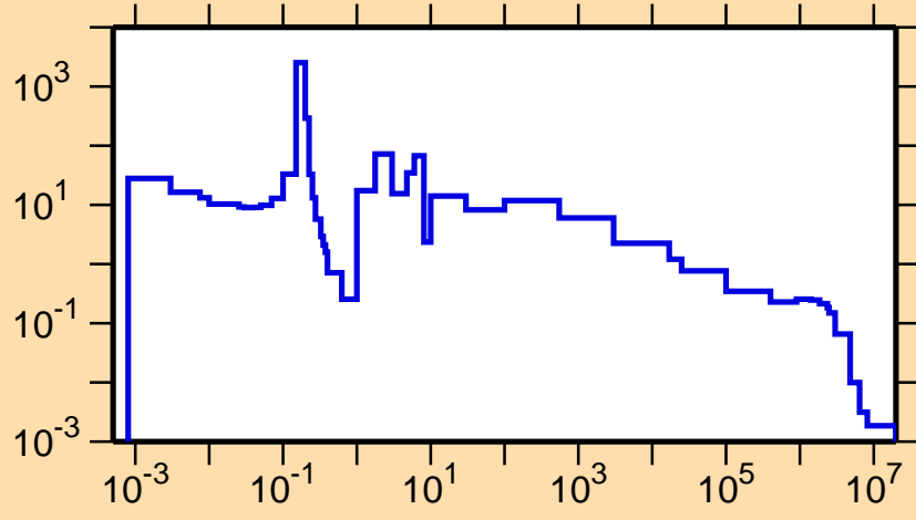
\sigma vs. E for ^{227}\text{Th}(n,\gamma)
