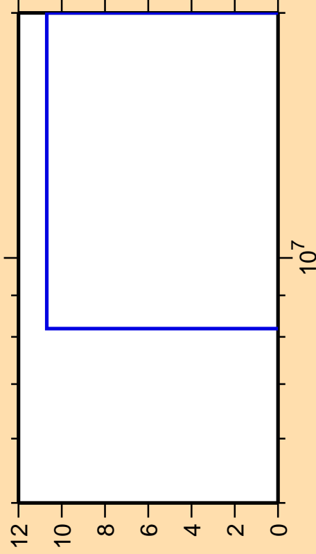
\Delta\sigma/\sigma vs. E for ^{227}\text{Th}(\text{mt117})
