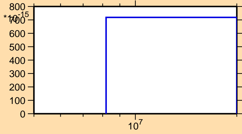
\sigma vs. E for ^{227}\text{Th} (mt 45)
