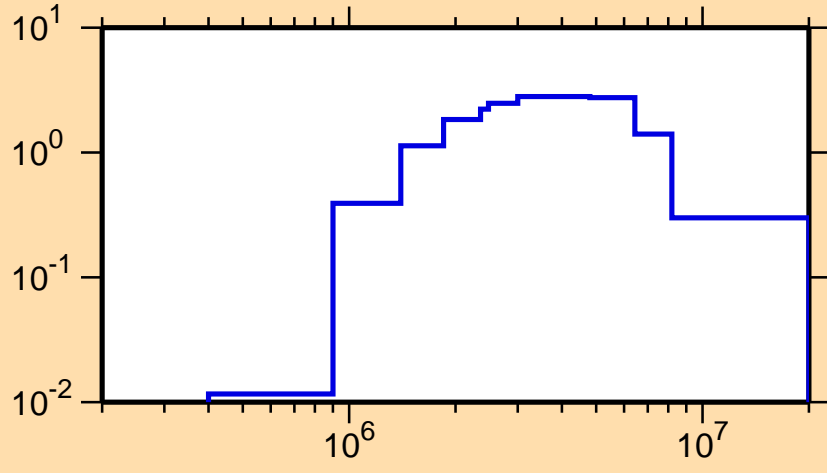
\sigma vs. E for ^{227}\text{Th}(n,n\text{cont.})
