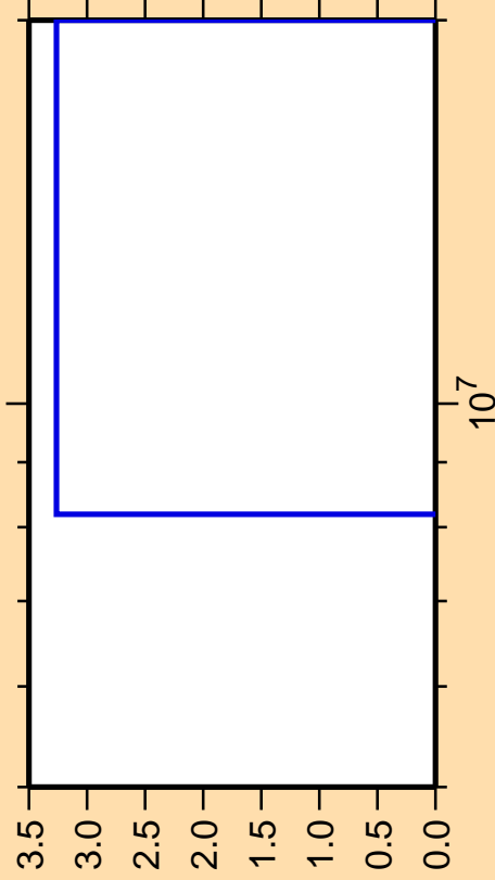
\Delta\sigma/\sigma vs. E for ^{227}\text{Th} (mt 45)
