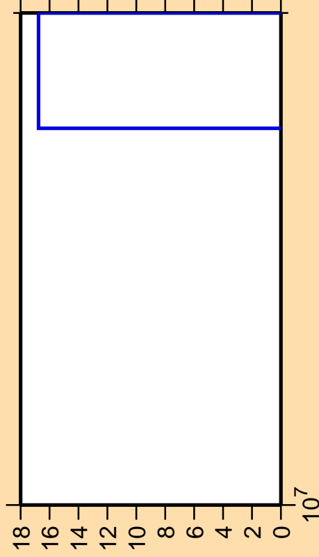
\Delta\sigma/\sigma vs. E for ^{228}\text{Th} (mt 45)
