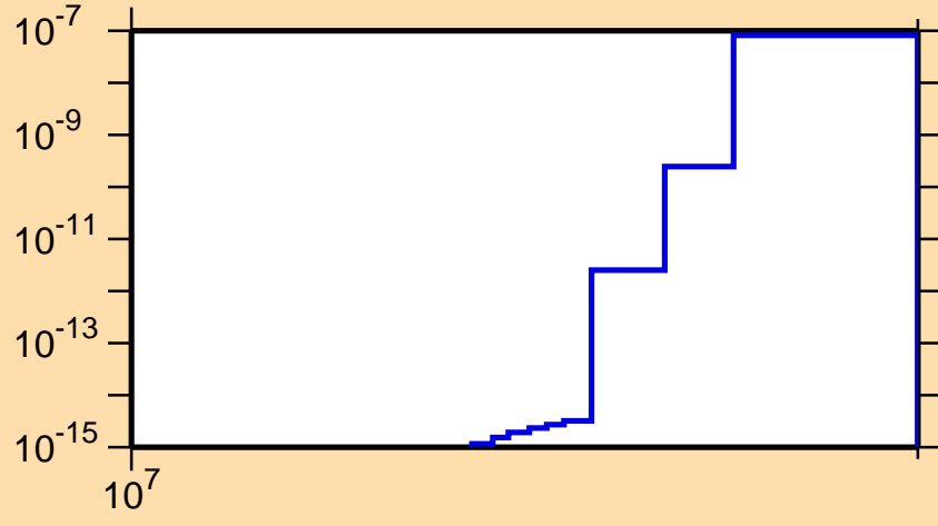
\sigma vs. E for ^{228}\text{Th}(n,2np)
