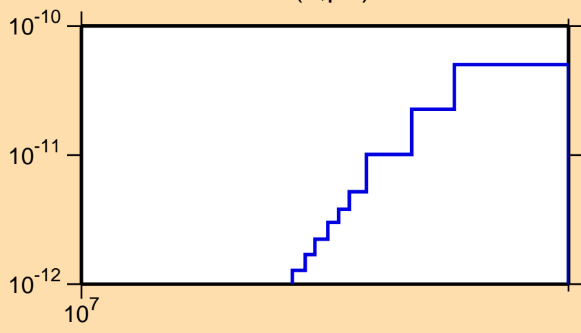
\sigma vs. E for ^{228}\text{Th}(n,p\alpha)
