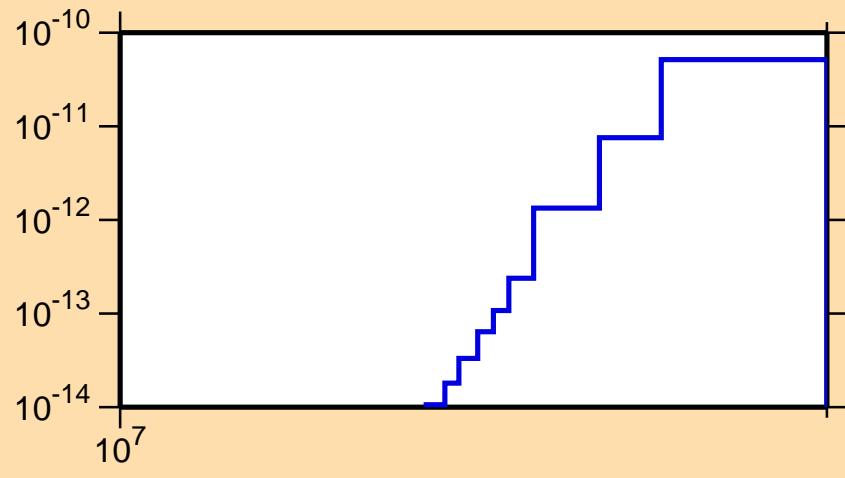
\sigma vs. E for ^{228}\text{Th}(\text{mt117})
