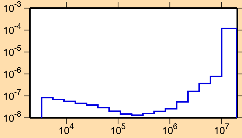
\sigma vs. E for ^{230}\text{Th}(n,\alpha)
