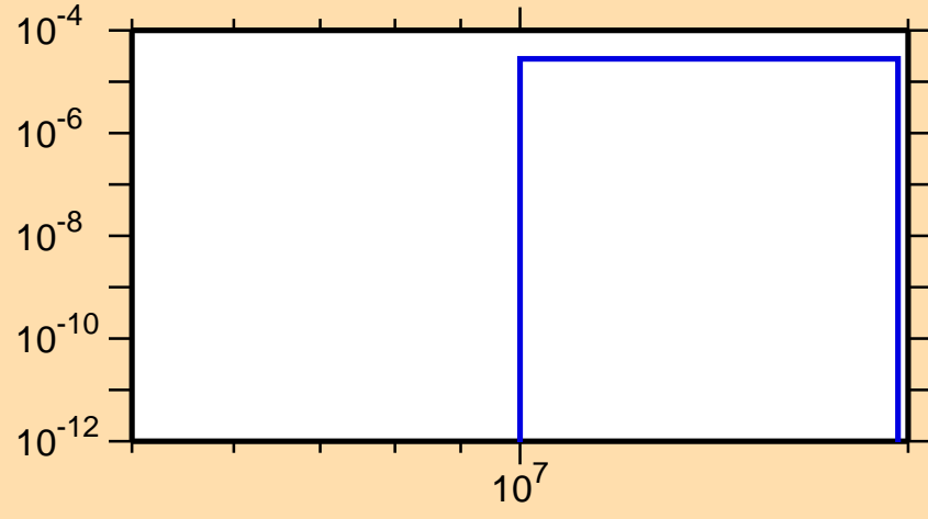
\sigma vs. E for ^{230}\text{Th}(n,np)
