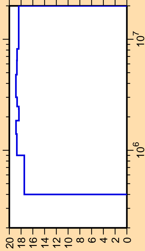
\Delta\sigma/\sigma vs. E for ^{230}\text{Th}(n,n_3)
