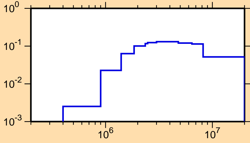
\sigma vs. E for ^{230}\text{Th}(n,n_3)
