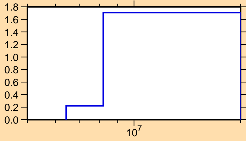
\sigma vs. E for ^{230}\text{Th}(n,2n)
