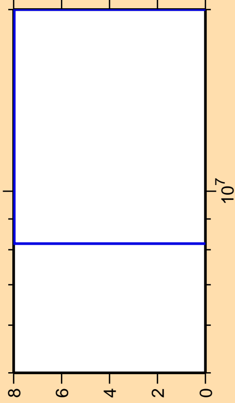
\Delta\sigma/\sigma vs. E for ^{230}\text{Th}(n,3n\alpha)
