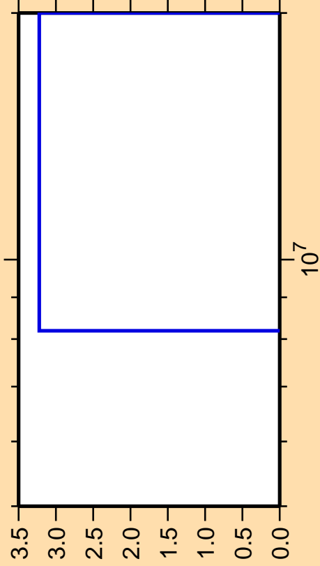
\Delta\sigma/\sigma vs. E for ^{230}\text{Th}(n,np)
