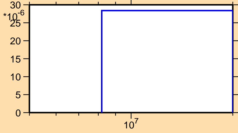
\sigma vs. E for ^{230}\text{Th}(n,d)
