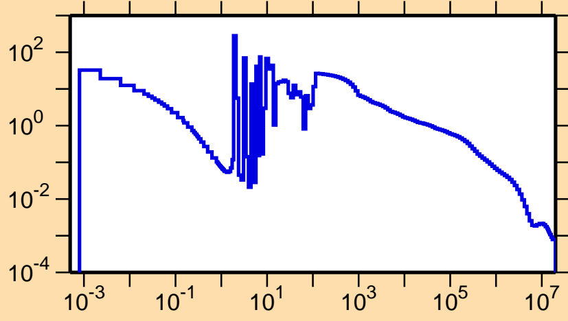
\sigma vs. E for ^{231}\text{Th}(n,\gamma)
