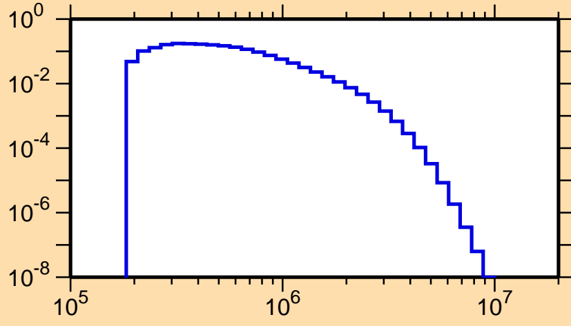
\sigma vs. E for ^{231}\text{Th}(n,n_4)
