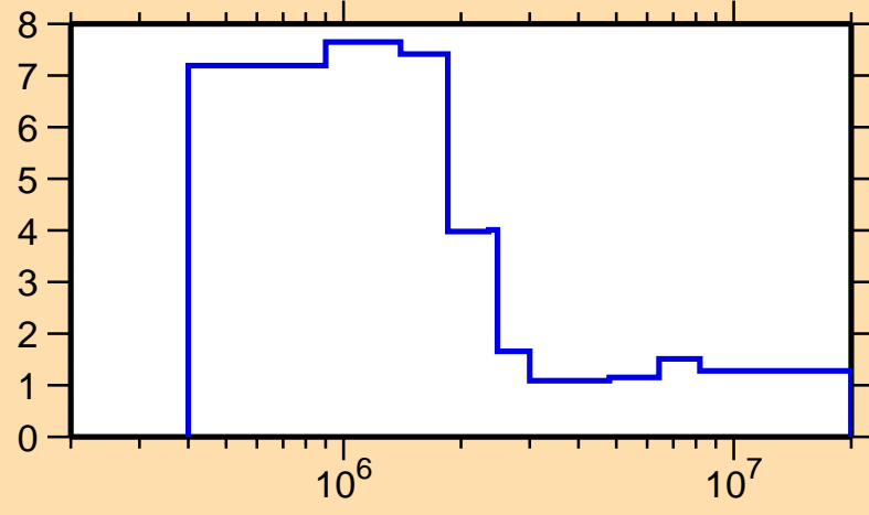
\Delta\sigma/\sigma vs. E for ^{231}\text{Th}(n, n_{\text{onel}})
