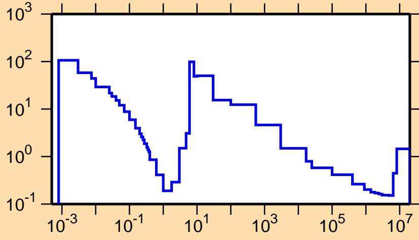
\sigma vs. E for ^{231}\text{Th}(n,f)
