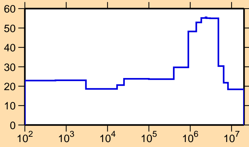
\Delta\sigma/\sigma vs. E for ^{231}\text{Th}(n,\gamma)
