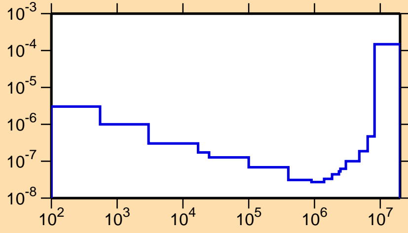
\sigma vs. E for ^{231}\text{Th}(n,\alpha)
