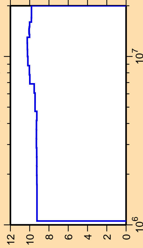
\Delta\sigma/\sigma vs. E for ^{232}\text{Th}(n,\text{ncont.})
