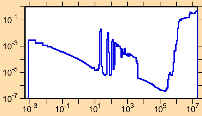
\sigma vs. E for ^{232}\text{Th}(n,f)
