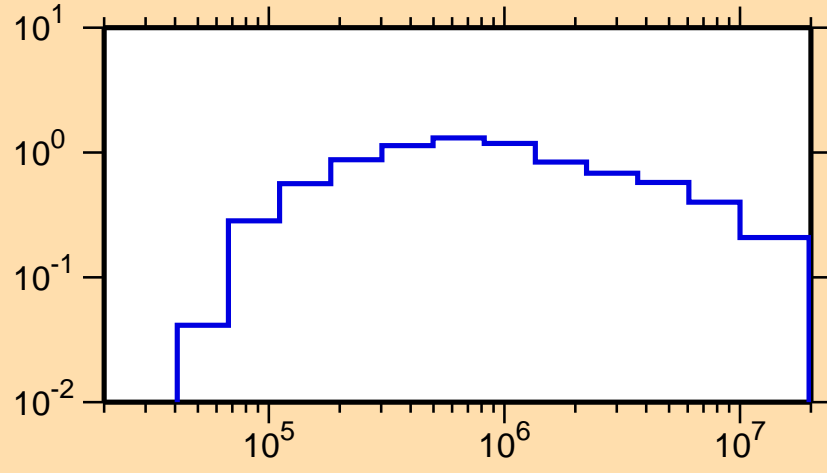
\sigma vs. E for ^{232}\text{Th}(n,n_1)
