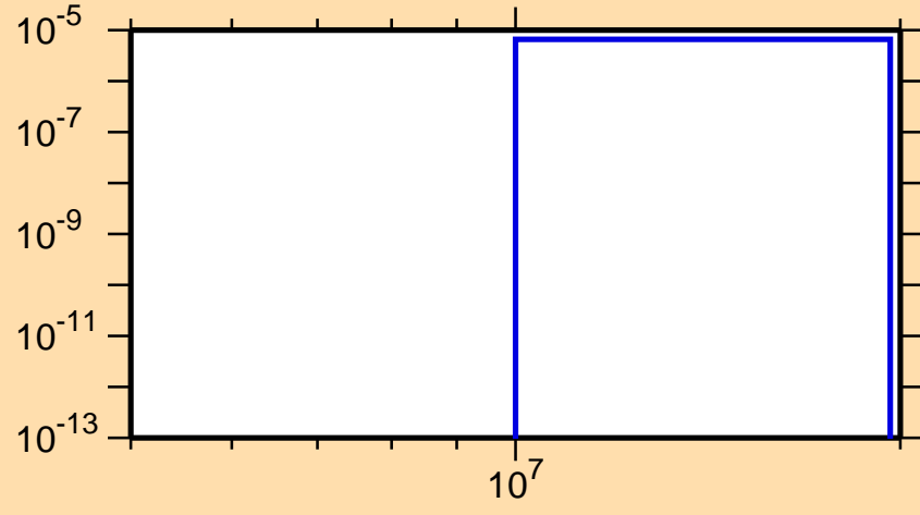
\sigma vs. E for ^{232}\text{Th}(n,t)
