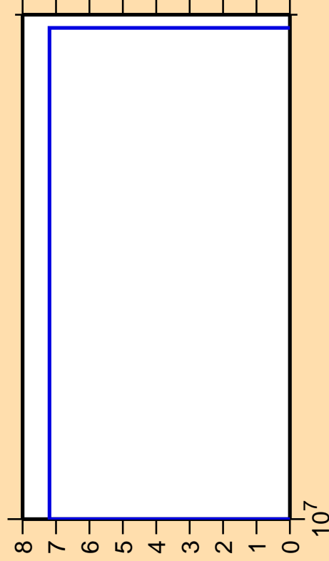
\Delta\sigma/\sigma vs. E for ^{232}\text{Th}(n,3n\alpha)
