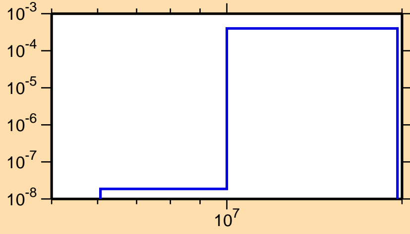
\sigma vs. E for ^{232}\text{Th}(n,p)
