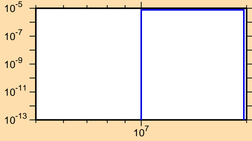
\sigma vs. E for ^{232}\text{Th}(n,np)
