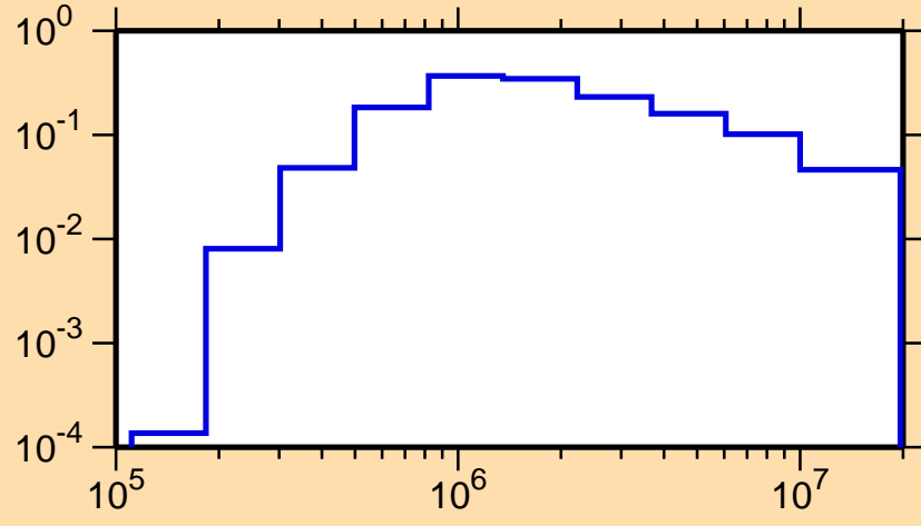
\sigma vs. E for ^{232}\text{Th}(n,n_2)
