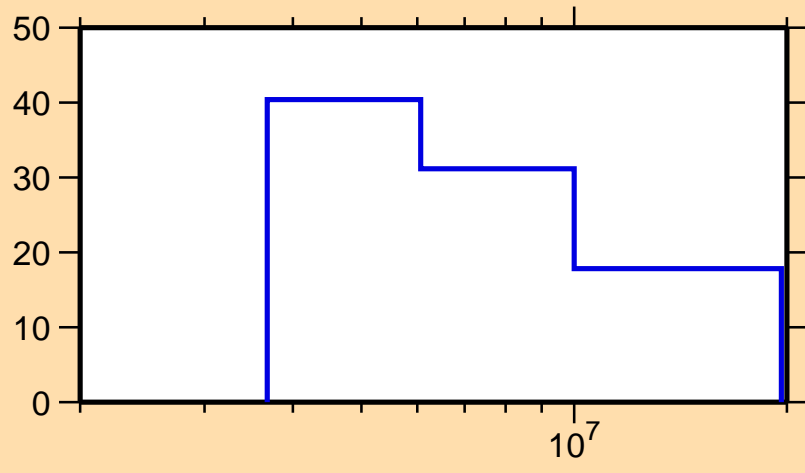
\Delta\sigma/\sigma vs. E for ^{233}\text{Th}(n,p)
