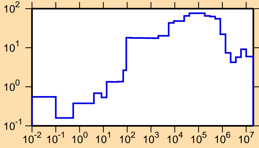
\Delta\sigma/\sigma vs. E for ^{233}\text{Th}(n,tot.)
