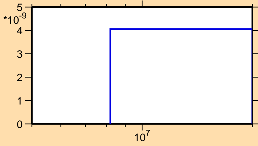
\sigma vs. E for ^{233}\text{Th}(n,\text{nd})
