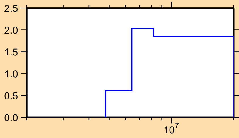
\sigma vs. E for ^{233}\text{Th}(n,2n)
