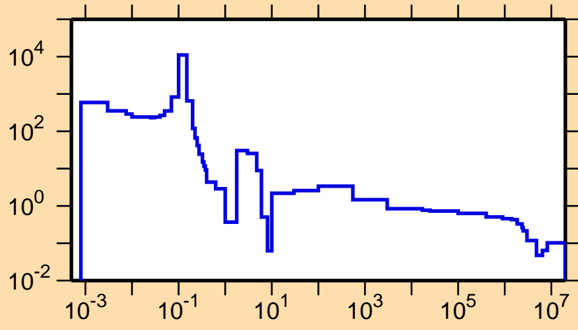
\sigma vs. E for ^{233}\text{Th}(n,f)
