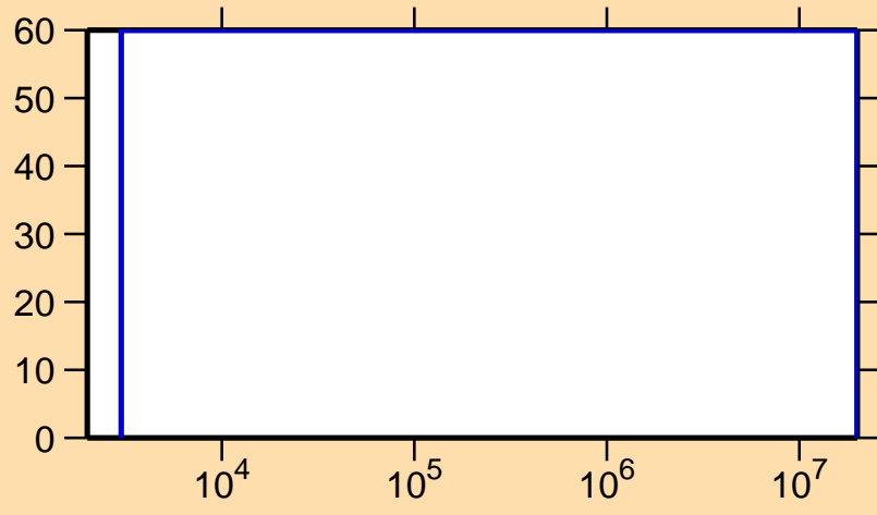
\Delta\sigma/\sigma vs. E for ^{233}\text{Th}(n,f)
