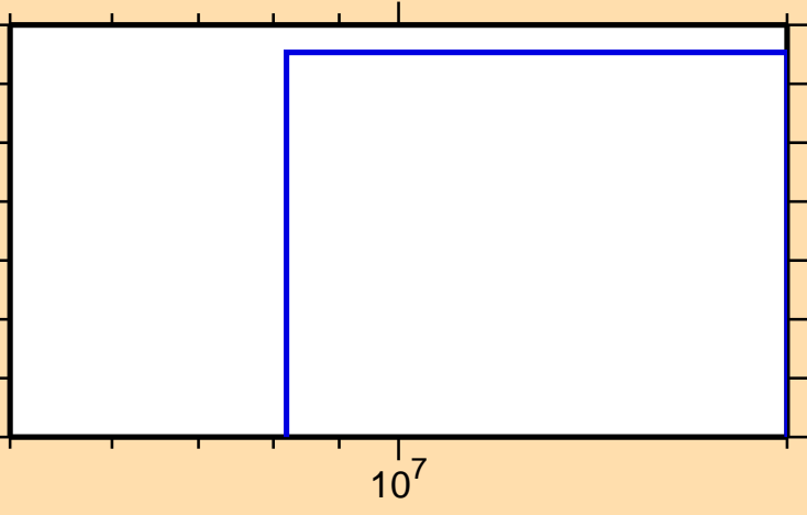
\sigma vs. E for ^{233}\text{Th}(n,t)
