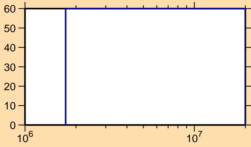
\Delta\sigma/\sigma vs. E for ^{234}\text{Th}(n,n_1)
