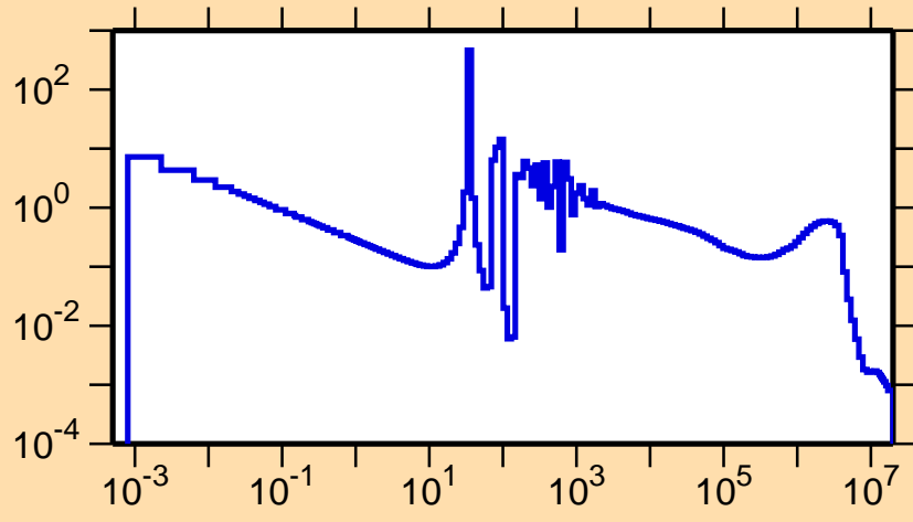
\sigma vs. E for ^{234}\text{Th}(n,\gamma)
