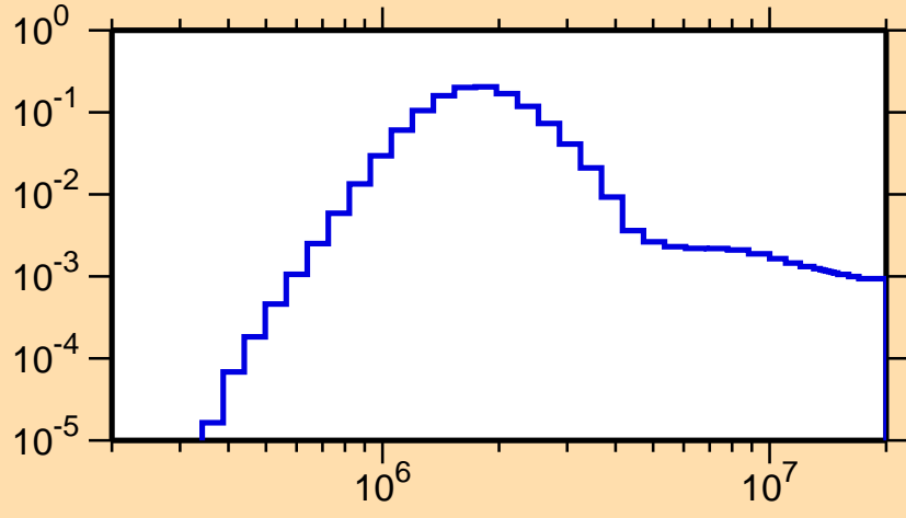
\sigma vs. E for ^{234}\text{Th}(n,n_3)
