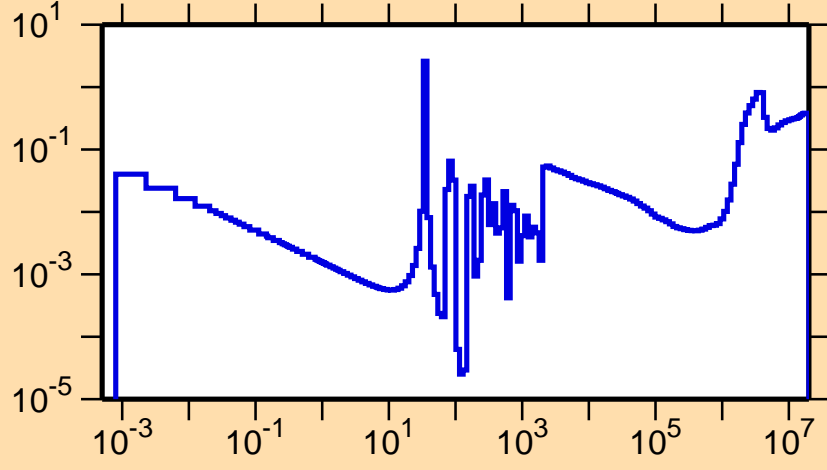
\sigma vs. E for ^{234}\text{Th}(n,f)
