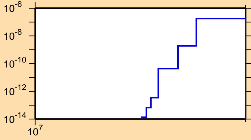
\sigma vs. E for ^{234}\text{Th}(n,nt)
