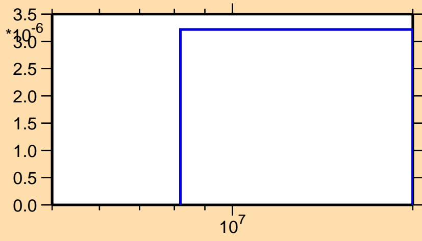
\sigma vs. E for ^{234}\text{Th}(n,np)
