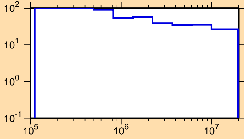
\Delta\sigma/\sigma vs. E for ^{235}\text{Th}(n,n\text{cont.})
