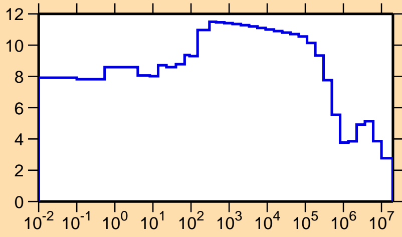
\sigma vs. E for ^{235}\text{Th}(n,\text{el.})
