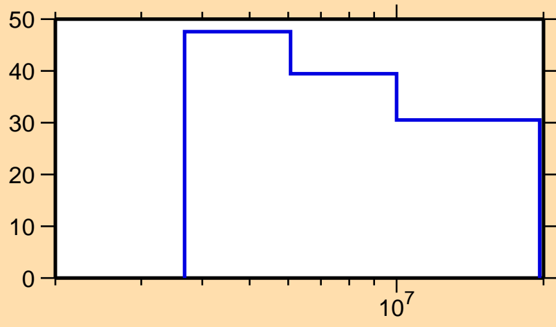
\Delta\sigma/\sigma vs. E for ^{235}\text{Th}(n,2n)
