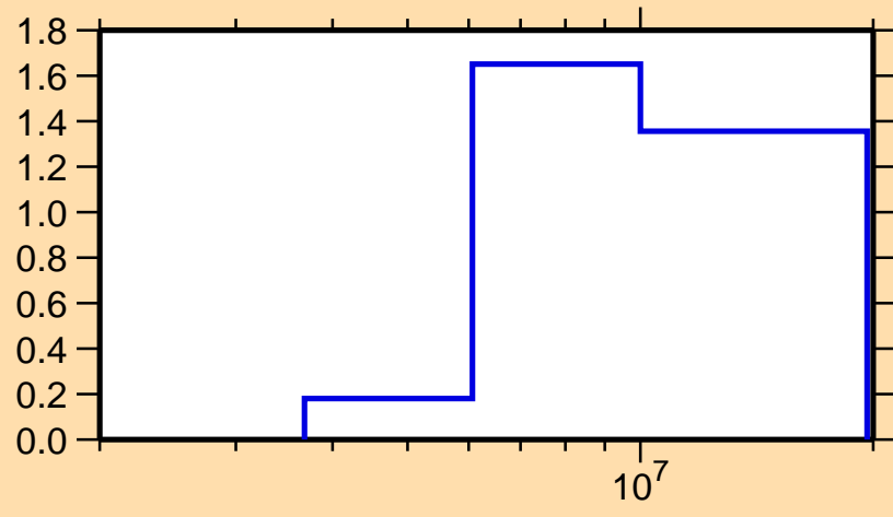
\sigma vs. E for ^{235}\text{Th}(n,2n)
