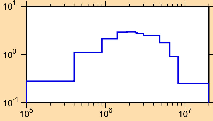
\sigma vs. E for ^{235}\text{Th}(n,\text{inel.})
