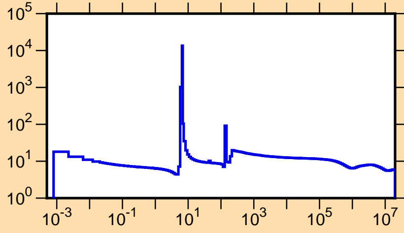
\sigma vs. E for ^{236}\text{Th}(n,\text{tot.})
