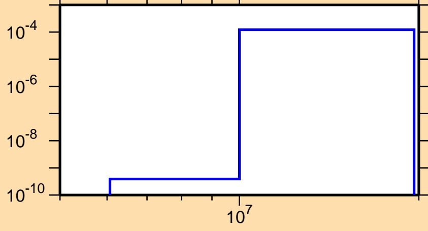
\sigma vs. E for ^{236}\text{Th}(n,p)
