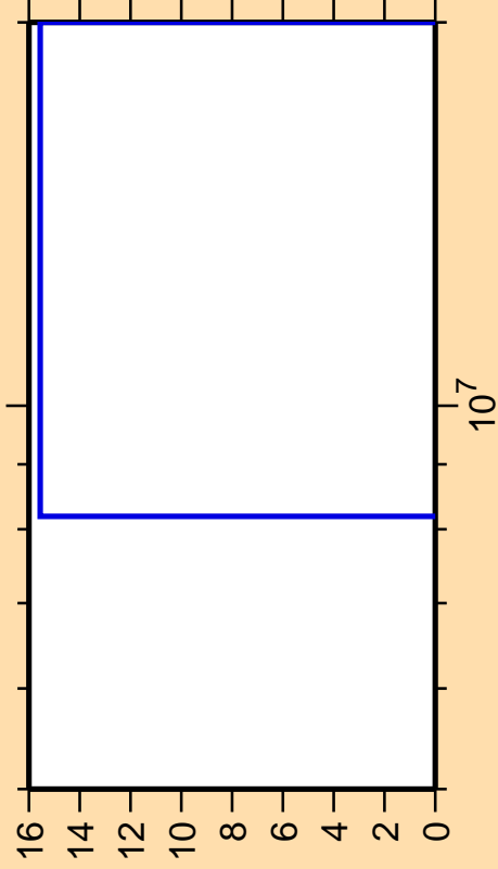
\Delta\sigma/\sigma vs. E for ^{236}\text{Th}(n,3n\alpha)
