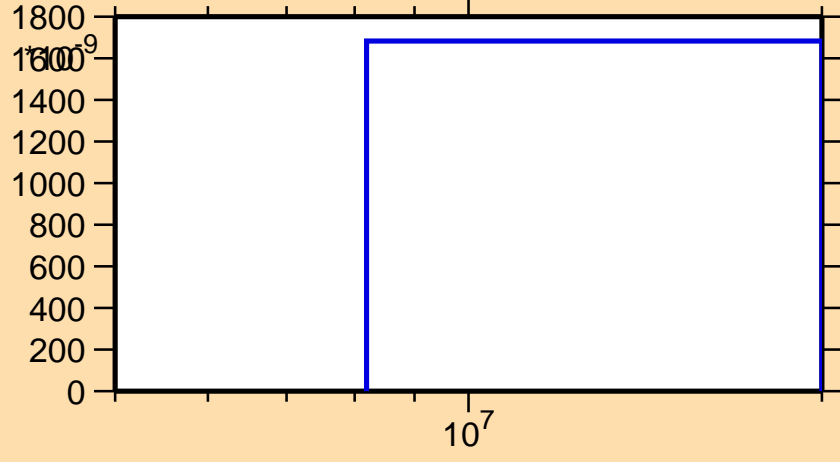
\sigma vs. E for ^{236}\text{Th}(n,np)
