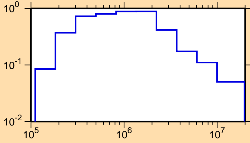
\sigma vs. E for ^{237}\text{Th}(n,n_1)
