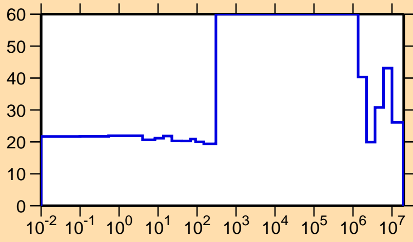
\Delta\sigma/\sigma vs. E for ^{237}\text{Th}(n,el.)
