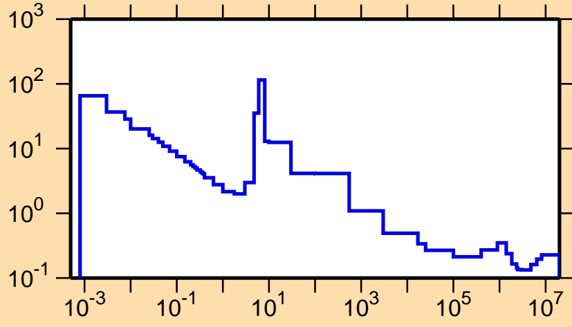
\sigma vs. E for ^{237}\text{Th}(n,f)
