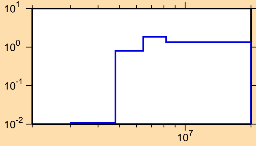
\sigma vs. E for ^{237}\text{Th}(n,2n)
