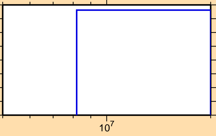
\sigma vs. E for ^{237}\text{Th}(n,t)
