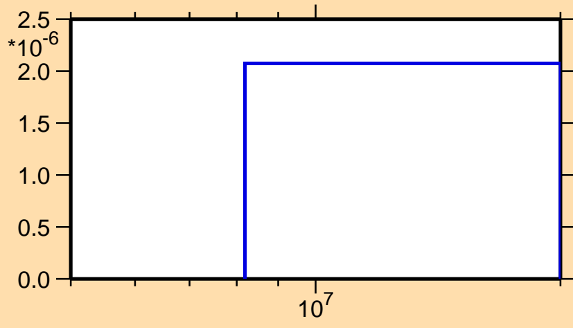
\sigma vs. E for ^{237}\text{Th}(n,np)
