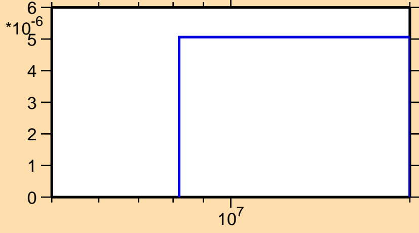
\sigma vs. E for ^{237}\text{Th}(n,d)
