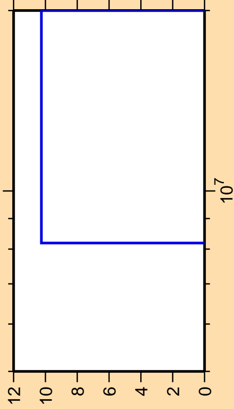
\Delta\sigma/\sigma vs. E for ^{237}\text{Th}(n,3n\alpha)
