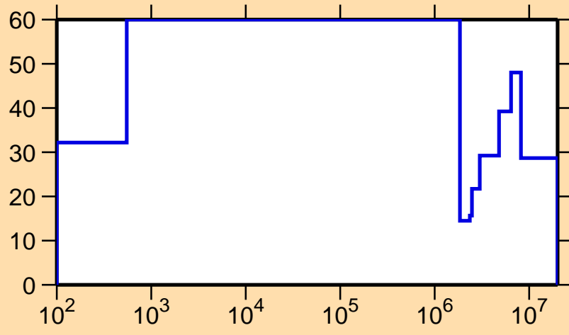
\Delta\sigma/\sigma vs. E for ^{237}\text{Th}(n,\text{el.})
