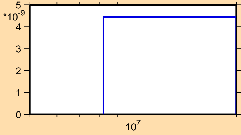
\sigma vs. E for ^{237}\text{Th}(n,nt)
