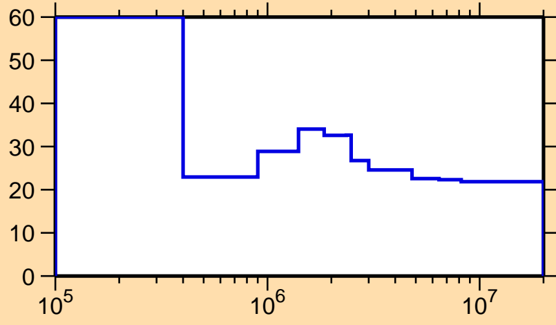
\Delta\sigma/\sigma vs. E for ^{237}\text{Th}(n,\text{nonel.})
