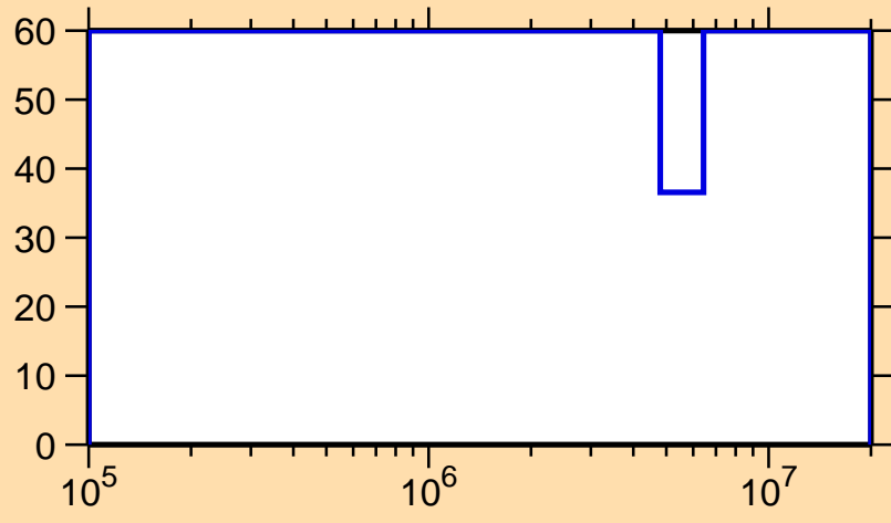
\Delta\sigma/\sigma vs. E for ^{237}\text{Th}(n,n\text{cont.})
