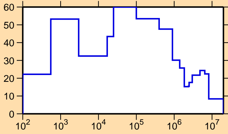
\Delta\sigma/\sigma vs. E for ^{237}\text{Th}(n,\text{tot.})
