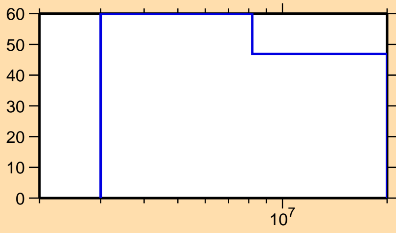
\Delta\sigma/\sigma vs. E for ^{237}\text{Th}(n,2n)
