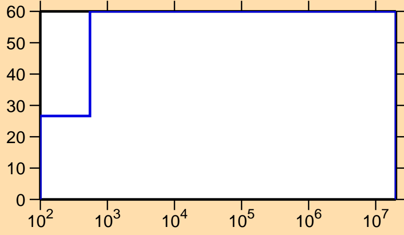
\Delta\sigma/\sigma vs. E for ^{237}\text{Th}(n,\gamma)
