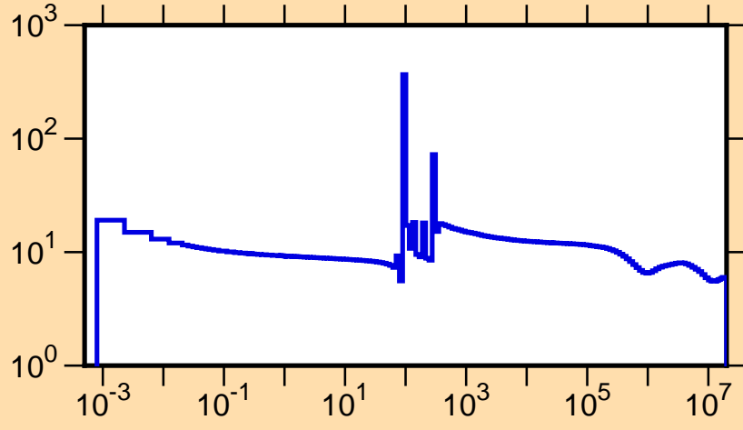
\sigma vs. E for ^{238}\text{Th}(n,\text{tot.})
