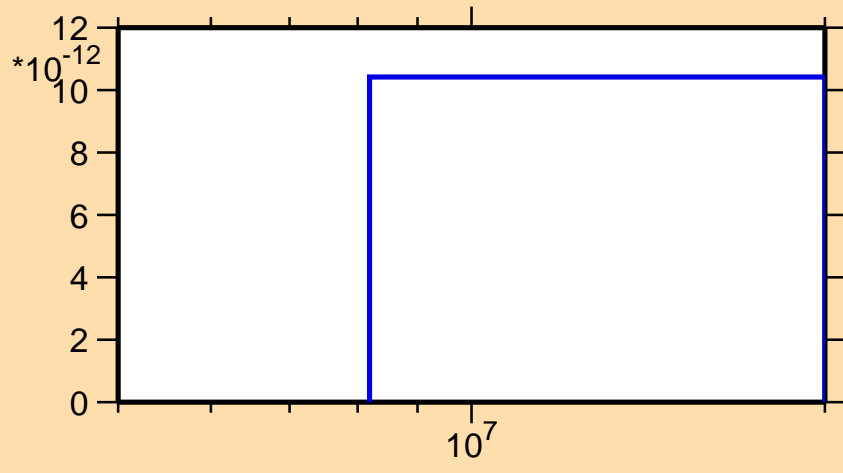
\sigma vs. E for ^{238}\text{Th}(n,3n\alpha)
