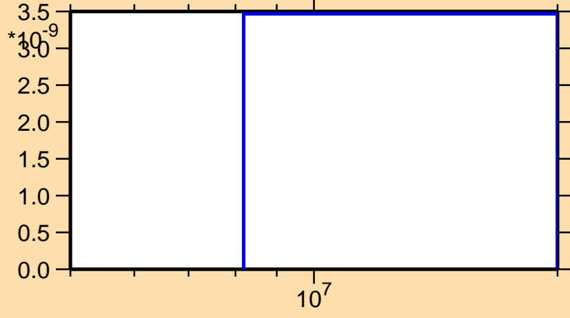
\sigma vs. E for ^{238}\text{Th}(n,nt)
