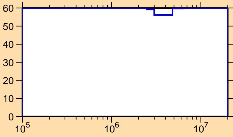
\Delta\sigma/\sigma vs. E for ^{238}\text{Th}(n,n_1)
