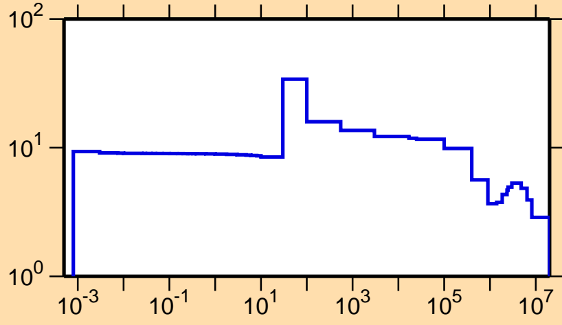
\sigma vs. E for ^{238}\text{Th}(n,\text{el.})
