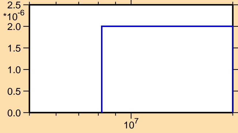
\sigma vs. E for ^{238}\text{Th}(n,np)
