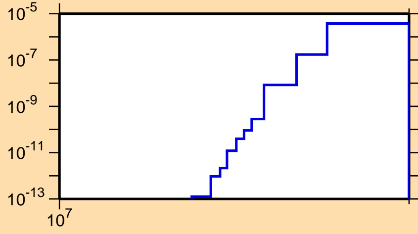
\sigma vs. E for ^{239}\text{Th}(n,nt)
