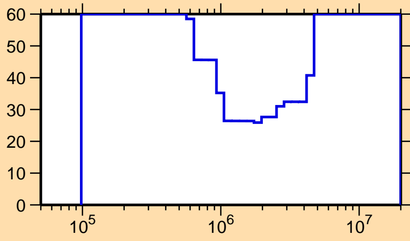
\Delta\sigma/\sigma vs. E for ^{239}\text{Th}(n,n\text{cont.})
