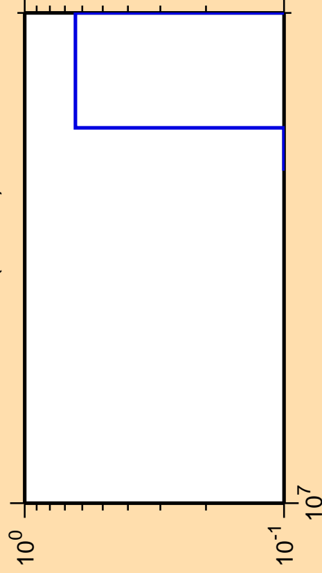
\Delta\sigma/\sigma vs. E for ^{239}\text{Th}(\text{mt } 11)
