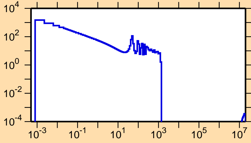
\sigma vs. E for ^{239}\text{Th}(n,f)
