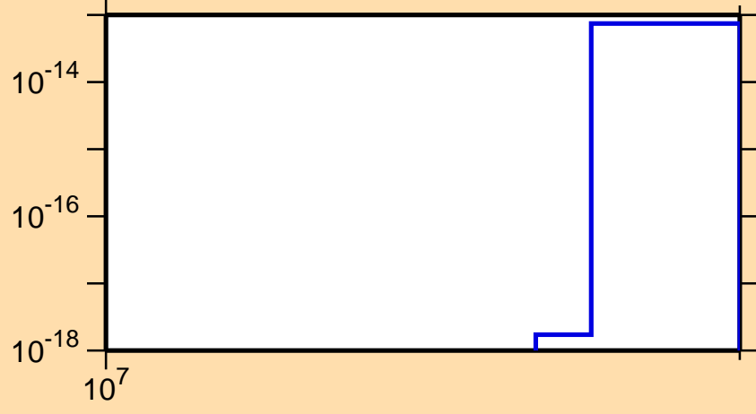
\sigma vs. E for ^{239}\text{Th}(\text{mt } 11)
