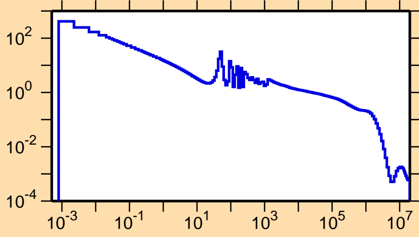
\sigma vs. E for ^{239}\text{Th}(n,\gamma)
