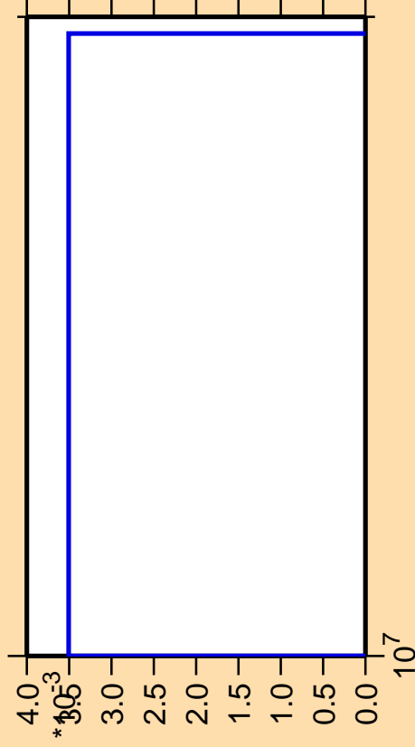
\Delta\sigma/\sigma vs. E for ^{239}\text{Th} (mt 11)
