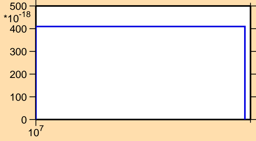
\sigma vs. E for ^{239}\text{Th} (mt 11)
