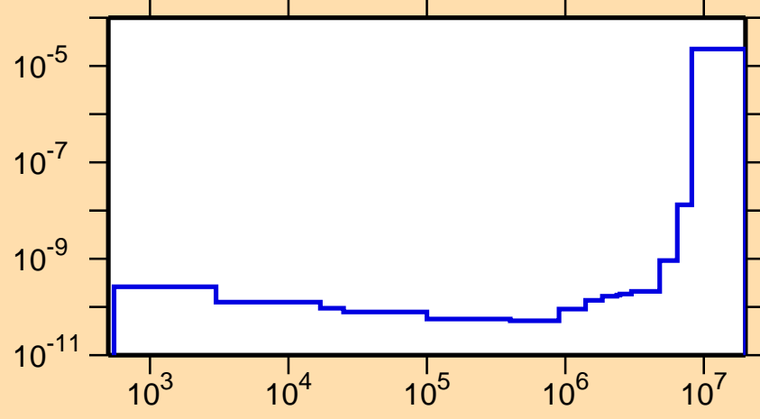
\sigma vs. E for ^{239}\text{Th}(n,\alpha)
