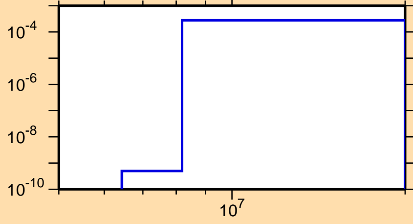
\sigma vs. E for ^{239}\text{Th}(n,p)
