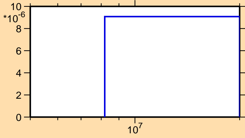
\sigma vs. E for ^{239}\text{Th}(n,d)
