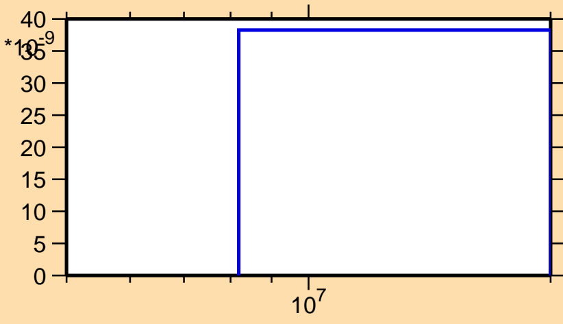
\sigma vs. E for ^{239}\text{Th}(n,nt)
