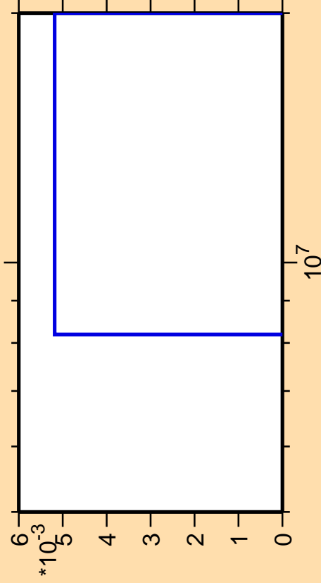
\Delta\sigma/\sigma vs. E for ^{239}\text{Th}(\text{mt } 11)
