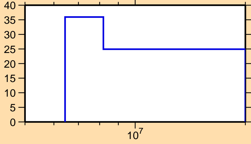
\Delta\sigma/\sigma vs. E for ^{239}\text{Th}(n,el.)
