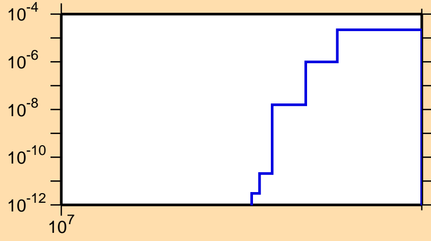
\sigma vs. E for ^{44}\text{Ti}(\text{mt117})
