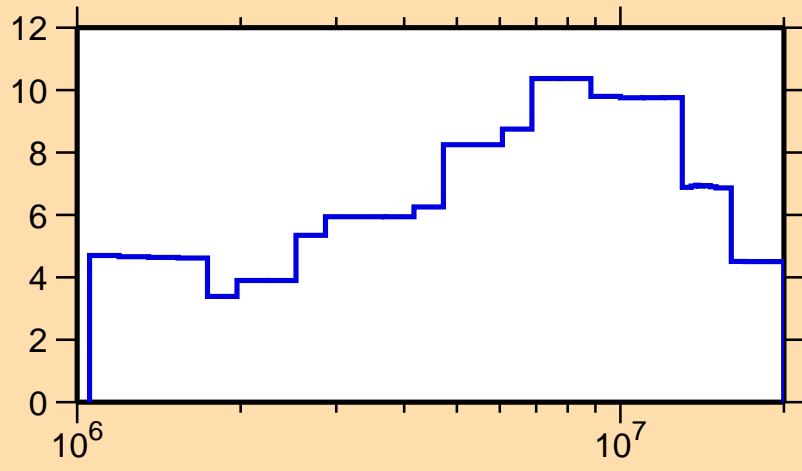
\Delta\sigma/\sigma vs. E for ^{44}\text{Ti}(n,\text{tot.})
