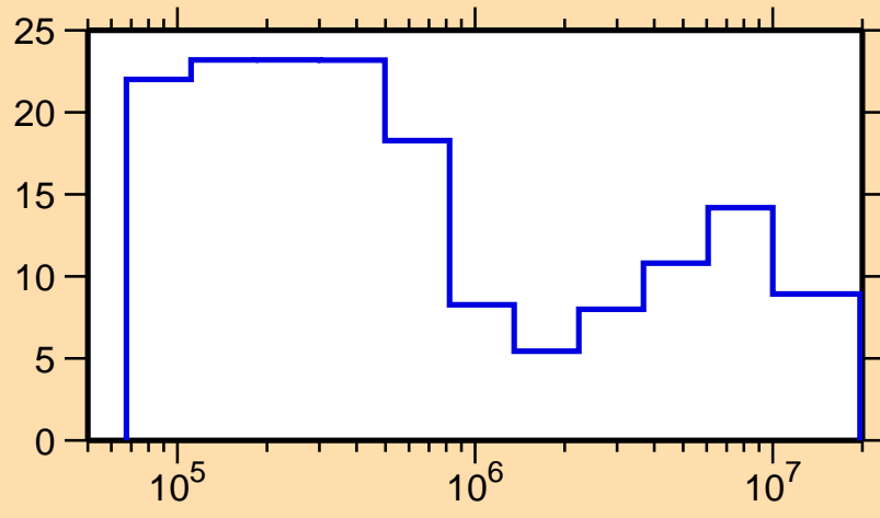
\Delta\sigma/\sigma vs. E for ^{44}\text{Ti}(n,el.)
