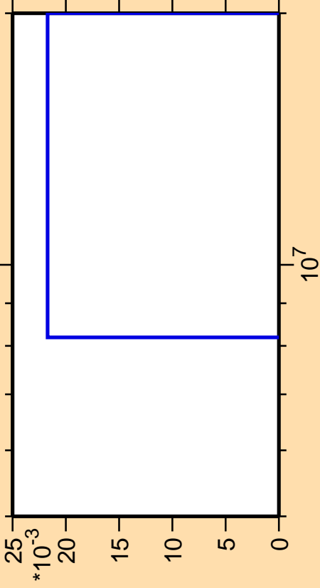
\Delta\sigma/\sigma vs. E for ^{44}\text{Ti} (mt 34)
