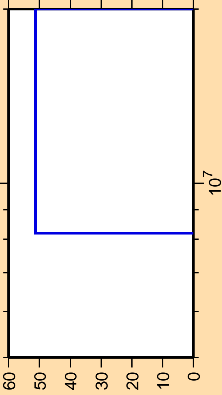
\Delta\sigma/\sigma vs. E for ^{44}\text{Ti}(n,2n)
