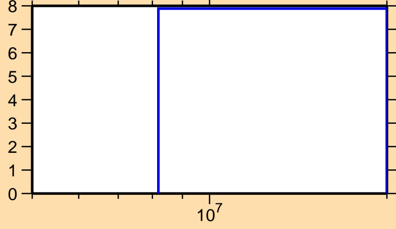
\Delta\sigma/\sigma vs. E for ^{44}\text{Ti}(n,\text{tot.})
