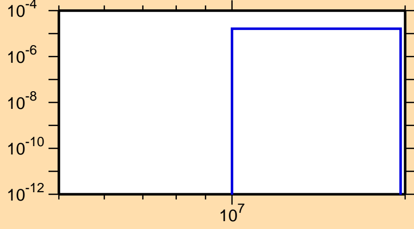
\sigma vs. E for ^{45}\text{Ti}(n,\text{He}3)
