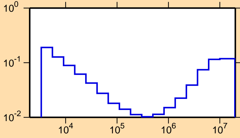
\sigma vs. E for ^{45}\text{Ti}(n,\alpha)
