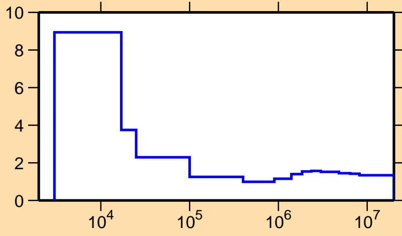
\sigma vs. E for ^{45}\text{Ti}(n,\text{nonel.})
