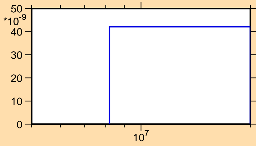
\sigma vs. E for ^{45}\text{Ti}(n,nd)
