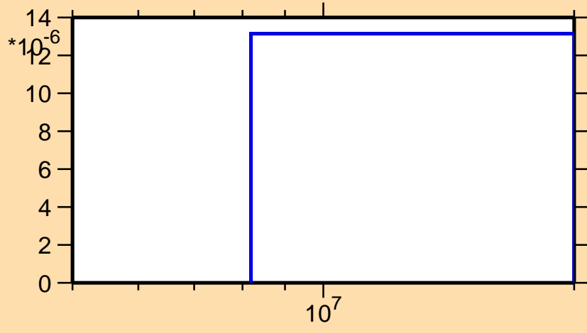
\sigma vs. E for ^{45}\text{Ti}(n,\text{He}3)
