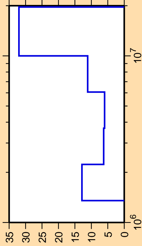
\Delta\sigma/\sigma vs. E for ^{46}\text{Ti}(n,n_2)
