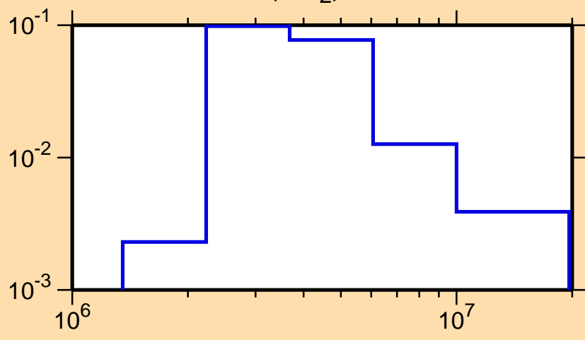
\sigma vs. E for ^{46}\text{Ti}(n,n_2)
