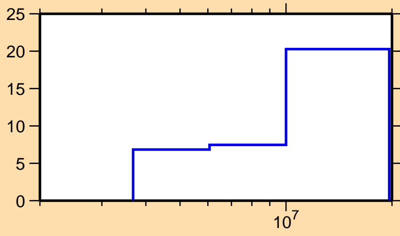
\Delta\sigma/\sigma vs. E for ^{46}\text{Ti}(n,n\text{cont.})
