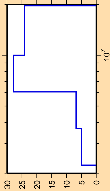
\Delta\sigma/\sigma vs. E for ^{46}\text{Ti}(n,n_4)
