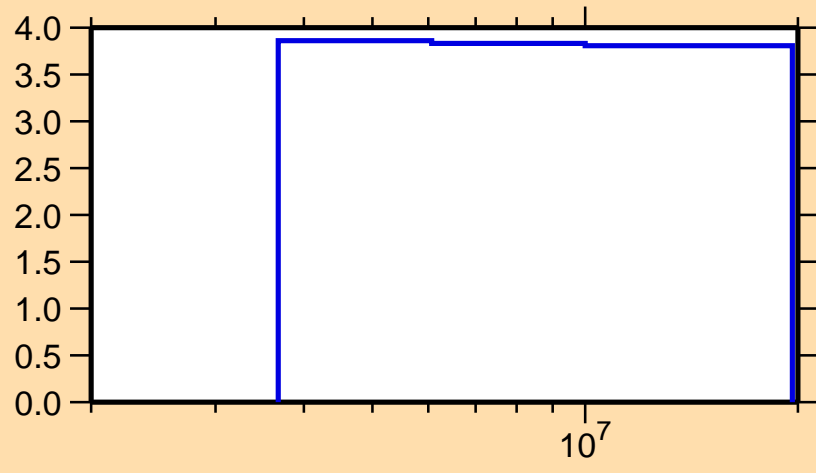
\Delta\sigma/\sigma vs. E for ^{46}\text{Ti}(n,n\text{onel.})
