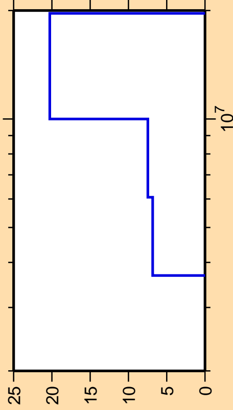
\Delta\sigma/\sigma vs. E for ^{46}\text{Ti}(n,\text{ncont.})
