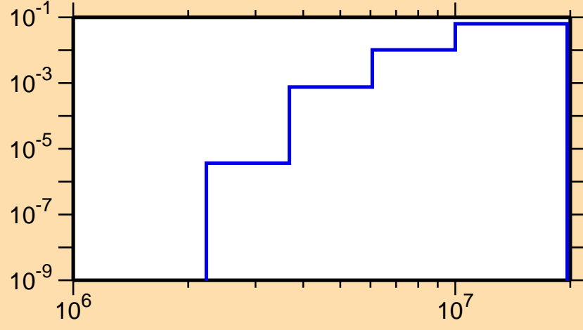
\sigma vs. E for ^{46}\text{Ti}(n,\alpha)
