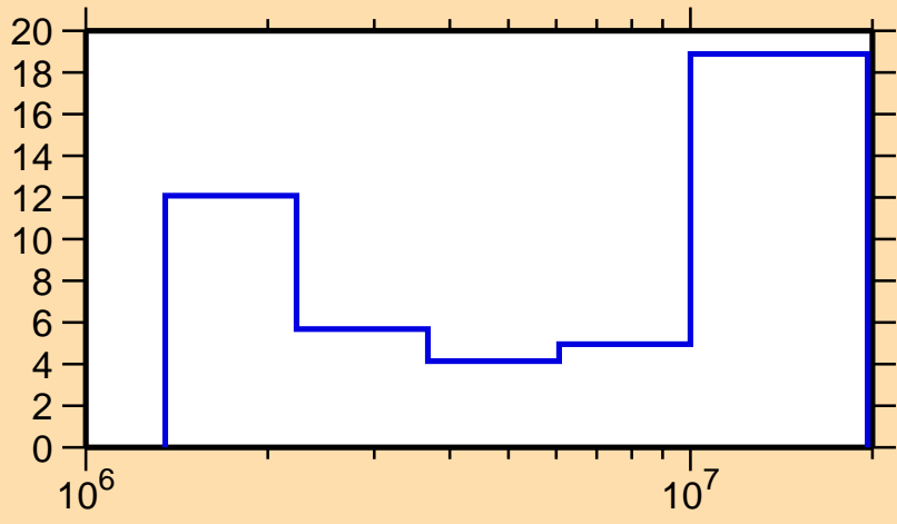
\Delta\sigma/\sigma vs. E for ^{46}\text{Ti}(n,\text{inel.})
