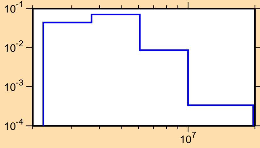
\sigma vs. E for ^{46}\text{Ti}(n,n_4)
