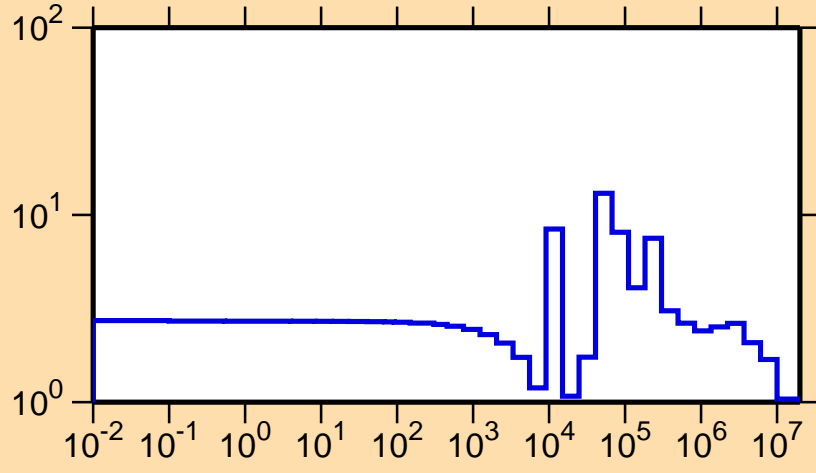
\sigma vs. E for ^{46}\text{Ti}(n,\text{el.})
