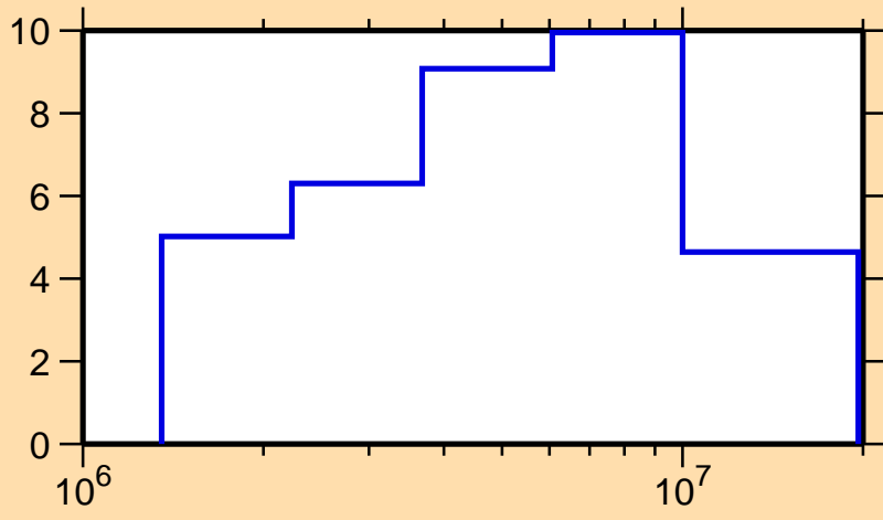
\Delta\sigma/\sigma vs. E for ^{46}\text{Ti}(n,el.)
