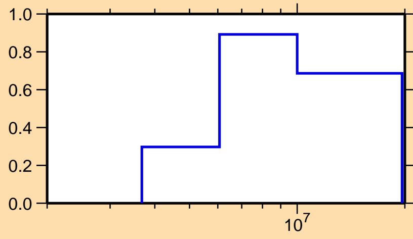
\sigma vs. E for ^{46}\text{Ti}(n,n\text{cont.})
