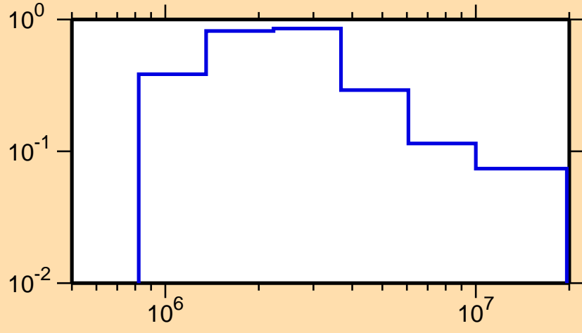
\sigma vs. E for ^{46}\text{Ti}(n,n_1)
