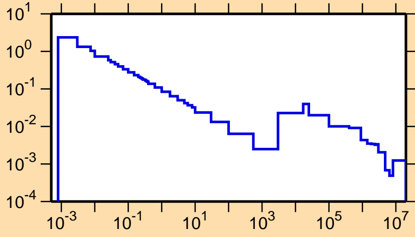
\sigma vs. E for ^{46}\text{Ti}(n,\gamma)
