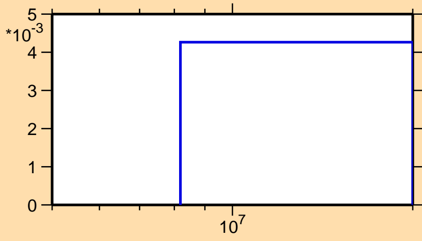
\sigma vs. E for ^{46}\text{Ti}(n,n\alpha)
