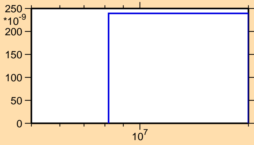
\sigma vs. E for ^{46}\text{Ti}(n,\text{He}3)
