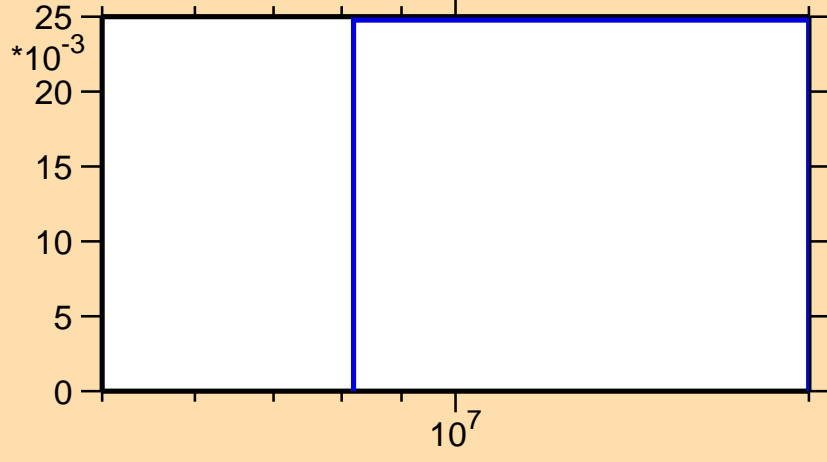
\sigma vs. E for ^{46}\text{Ti}(n,2n)
