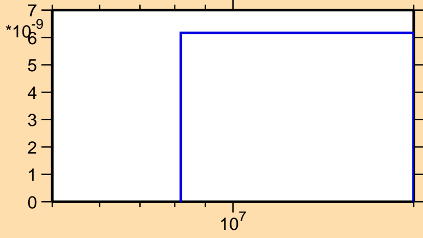
\sigma vs. E for ^{46}\text{Ti}(n,pd)
