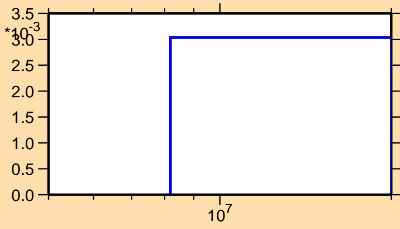
\sigma vs. E for ^{48}\text{Ti}(n,d)
