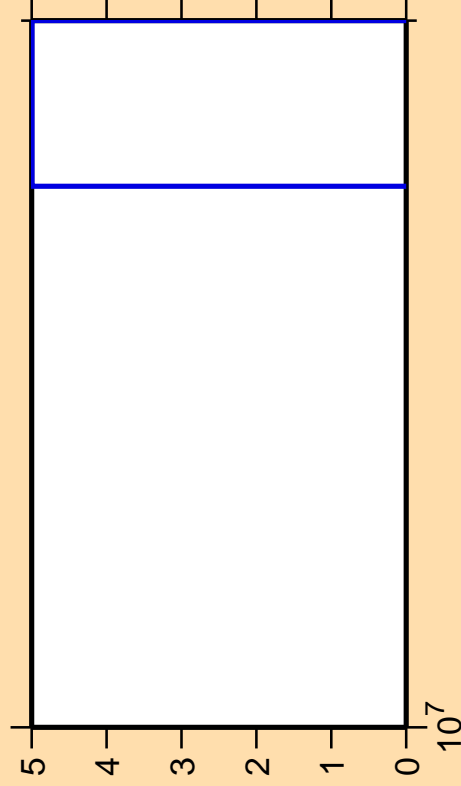
\Delta\sigma/\sigma vs. E for ^{48}\text{Ti}(n,2n\alpha)
