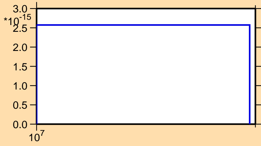
\sigma vs. E for ^{48}\text{Ti}(n,nt)
