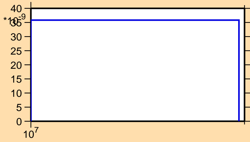
\sigma vs. E for ^{48}\text{Ti}(n,\text{nd})
