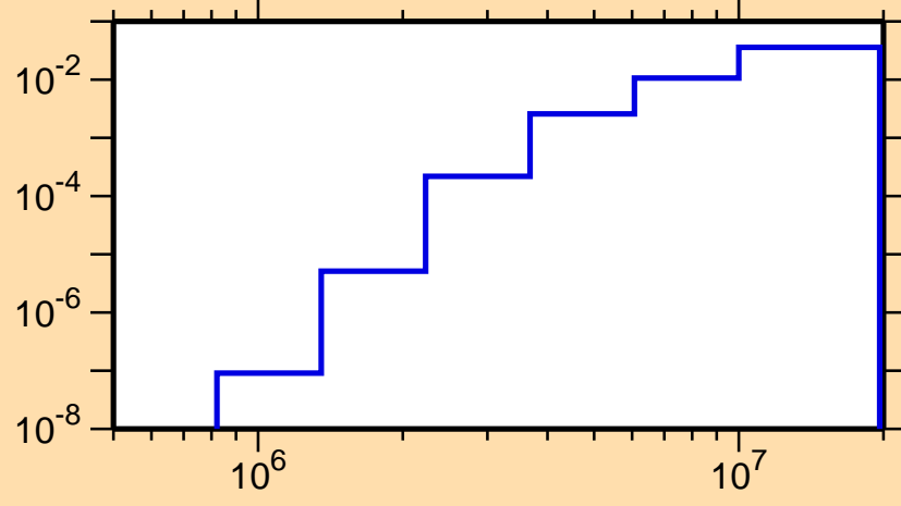
\sigma vs. E for ^{48}\text{Ti}(n,\alpha)
