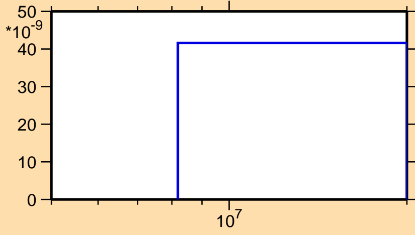
\sigma vs. E for ^{48}\text{Ti}(n,nd)
