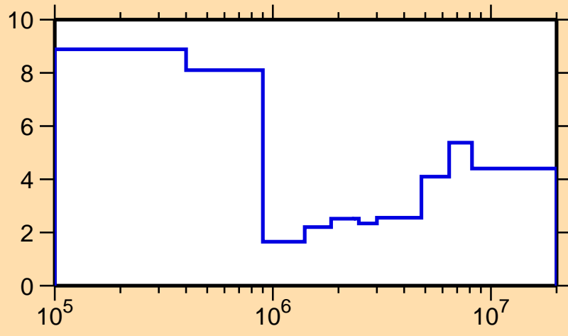
\Delta\sigma/\sigma vs. E for ^{48}\text{Ti}(n,el.)
