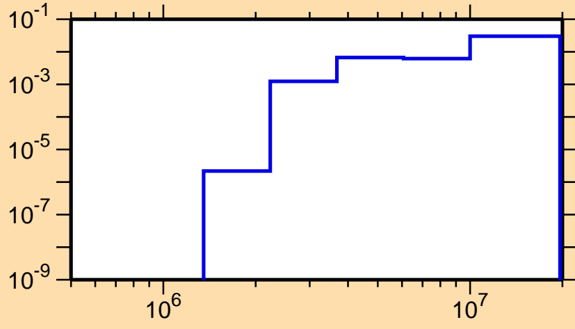
\sigma vs. E for ^{49}\text{Ti}(n,p)
