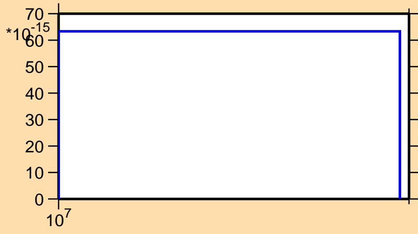
\sigma vs. E for ^{49}\text{Ti}(n,p\alpha)
