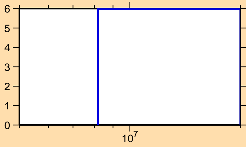
\Delta\sigma/\sigma vs. E for ^{49}\text{Ti}(n,\text{tot.})
