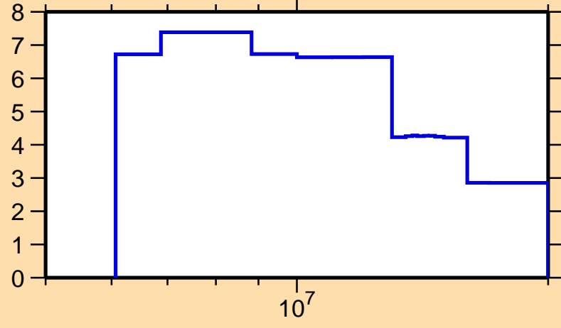
\Delta\sigma/\sigma vs. E for ^{50}\text{Ti}(n,tot.)
