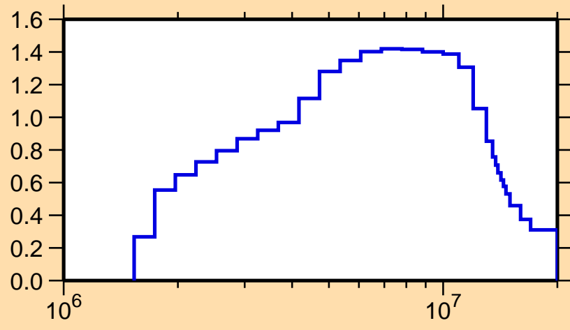
\sigma vs. E for ^{50}\text{Ti}(n,\text{inel.})
