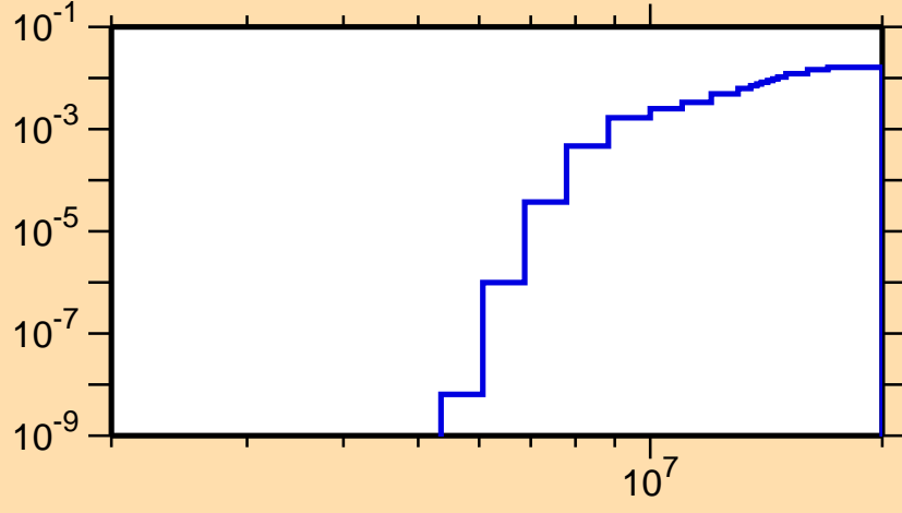
\sigma vs. E for ^{50}\text{Ti}(n,\alpha)
