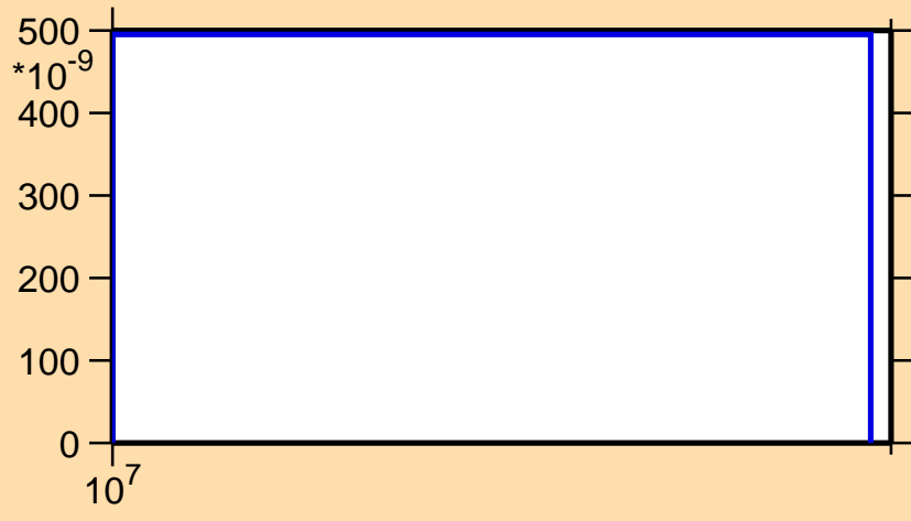
\sigma vs. E for ^{50}\text{Ti}(n,t)
