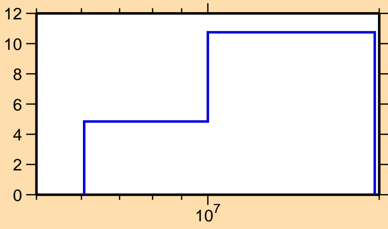
Δσ/σ vs. E for ^{50}\text{Ti}(n,\text{inel.})
