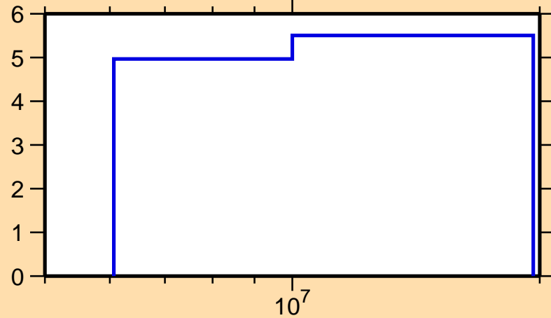
\Delta\sigma/\sigma vs. E for ^{50}\text{Ti}(n,\text{nonel.})
