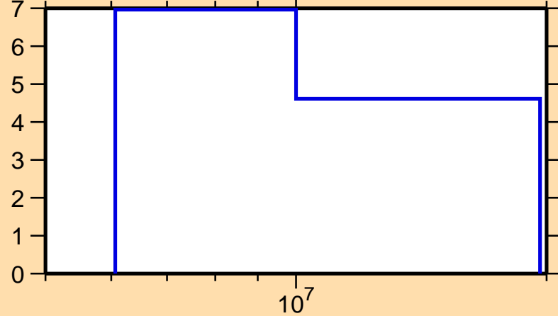
\Delta\sigma/\sigma vs. E for ^{50}\text{Ti}(n,\text{tot.})
