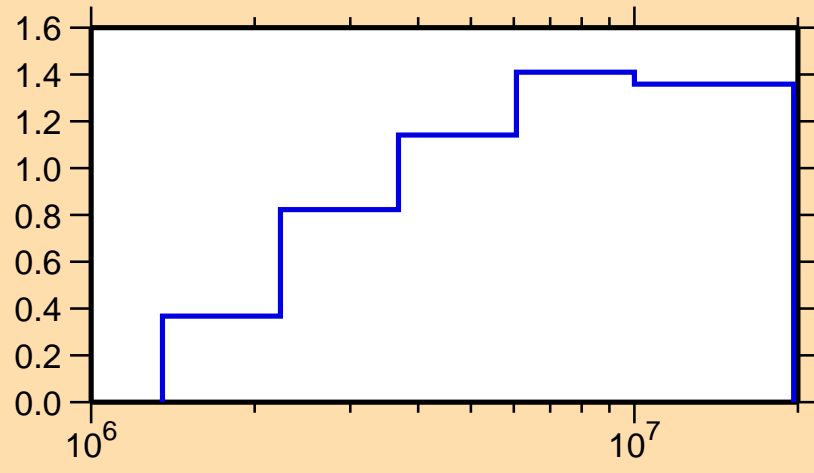
\sigma vs. E for ^{50}\text{Ti}(n,\text{nonel.})
